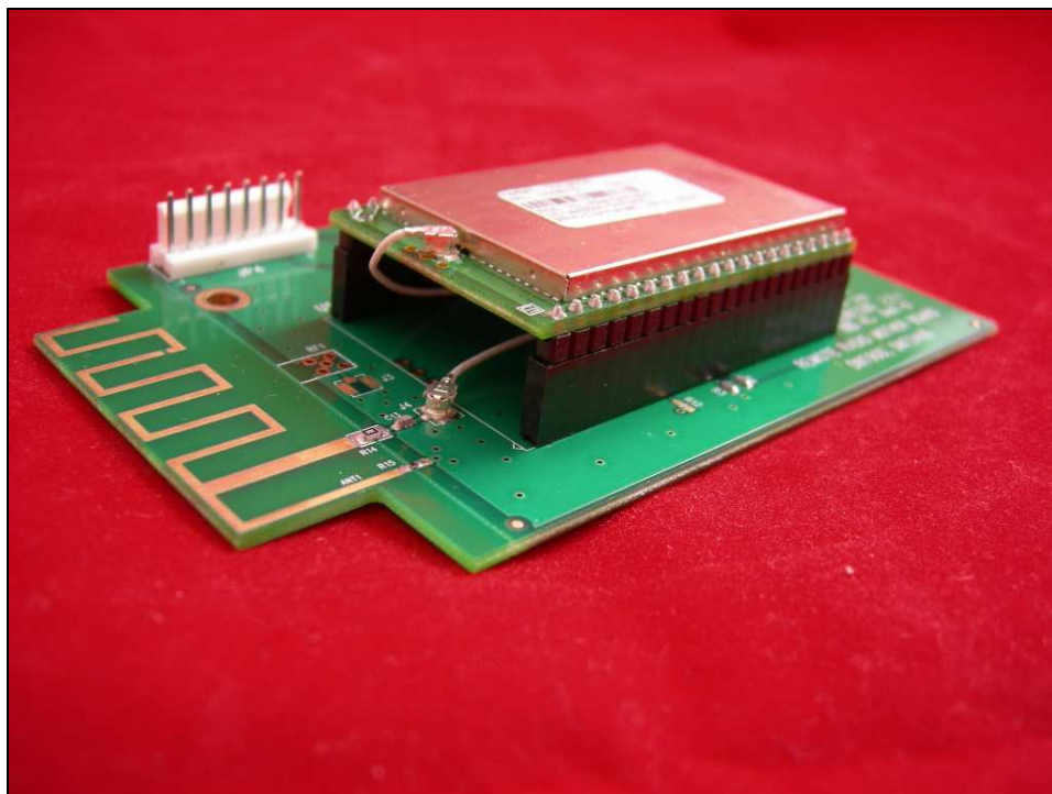
Figure 2: PCB - Front
