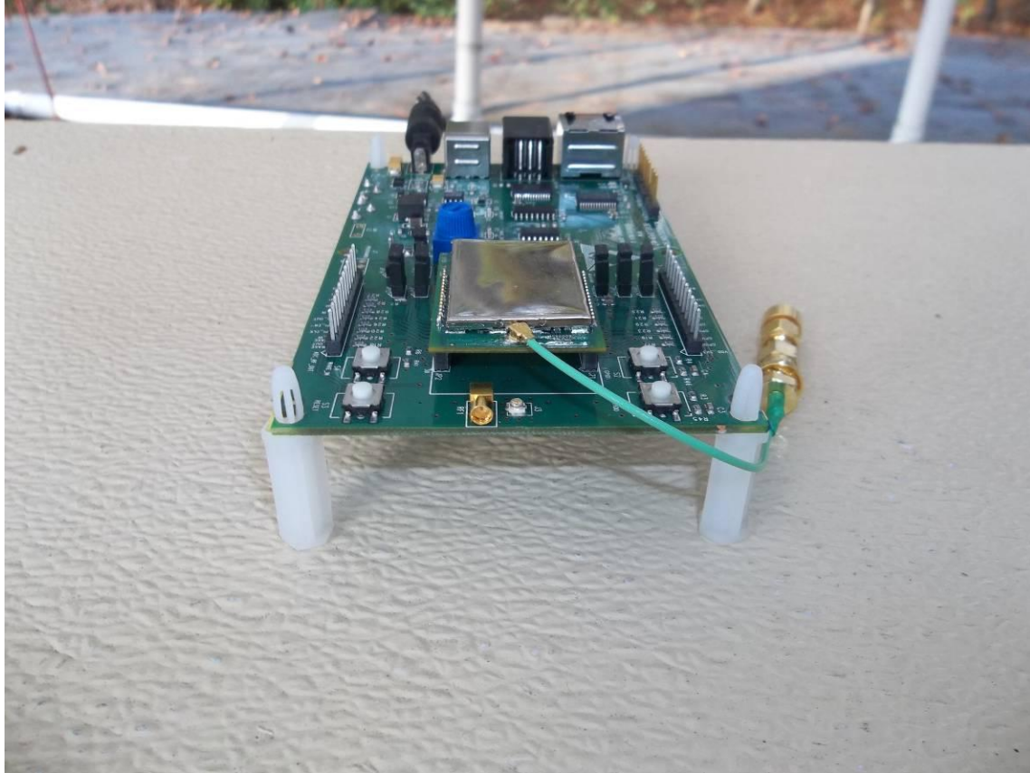
Figure 2. Radiated Emissions Test Setup, Front View Close Up
