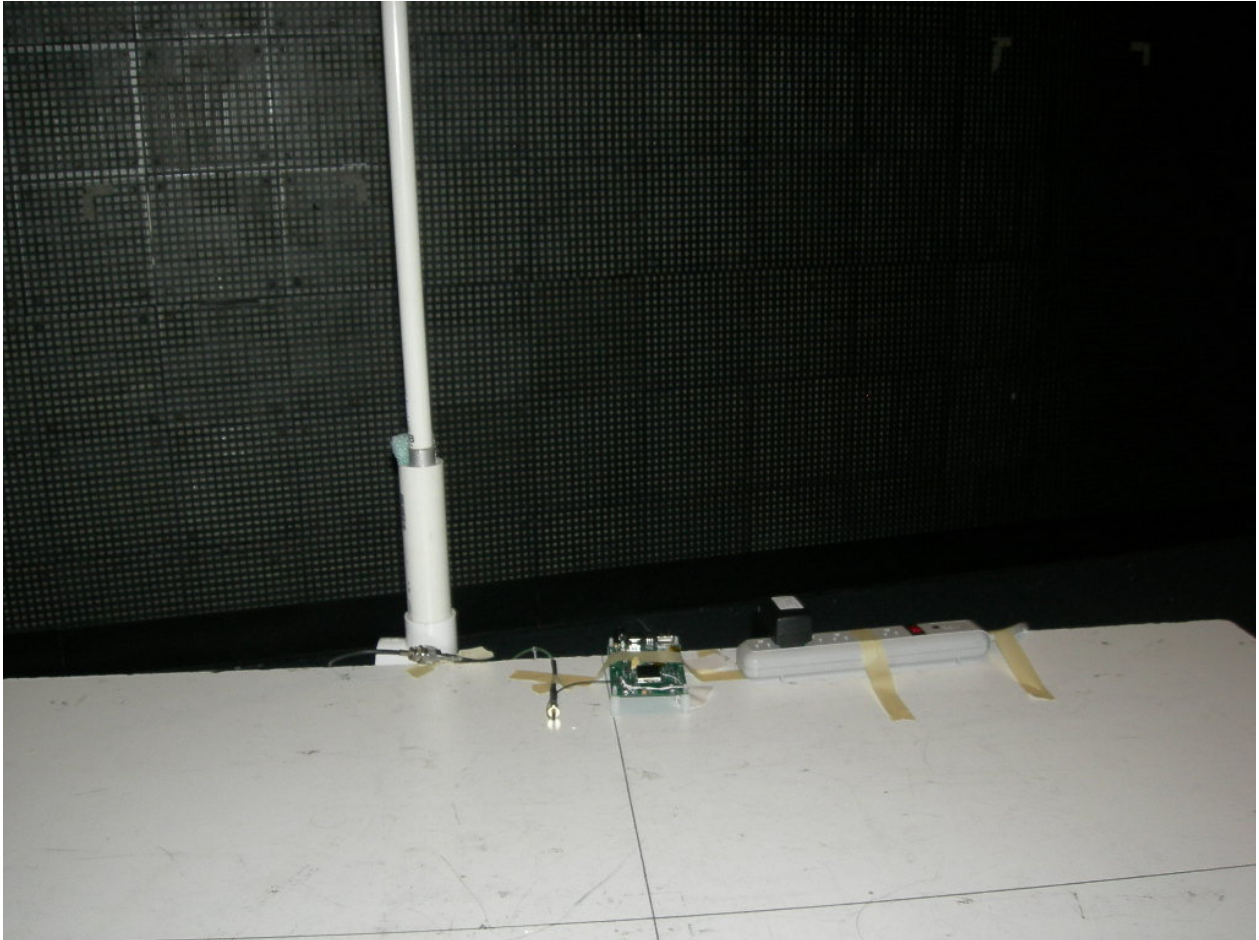
Figure 2: Radiated Emissions – Dipole Antenna
