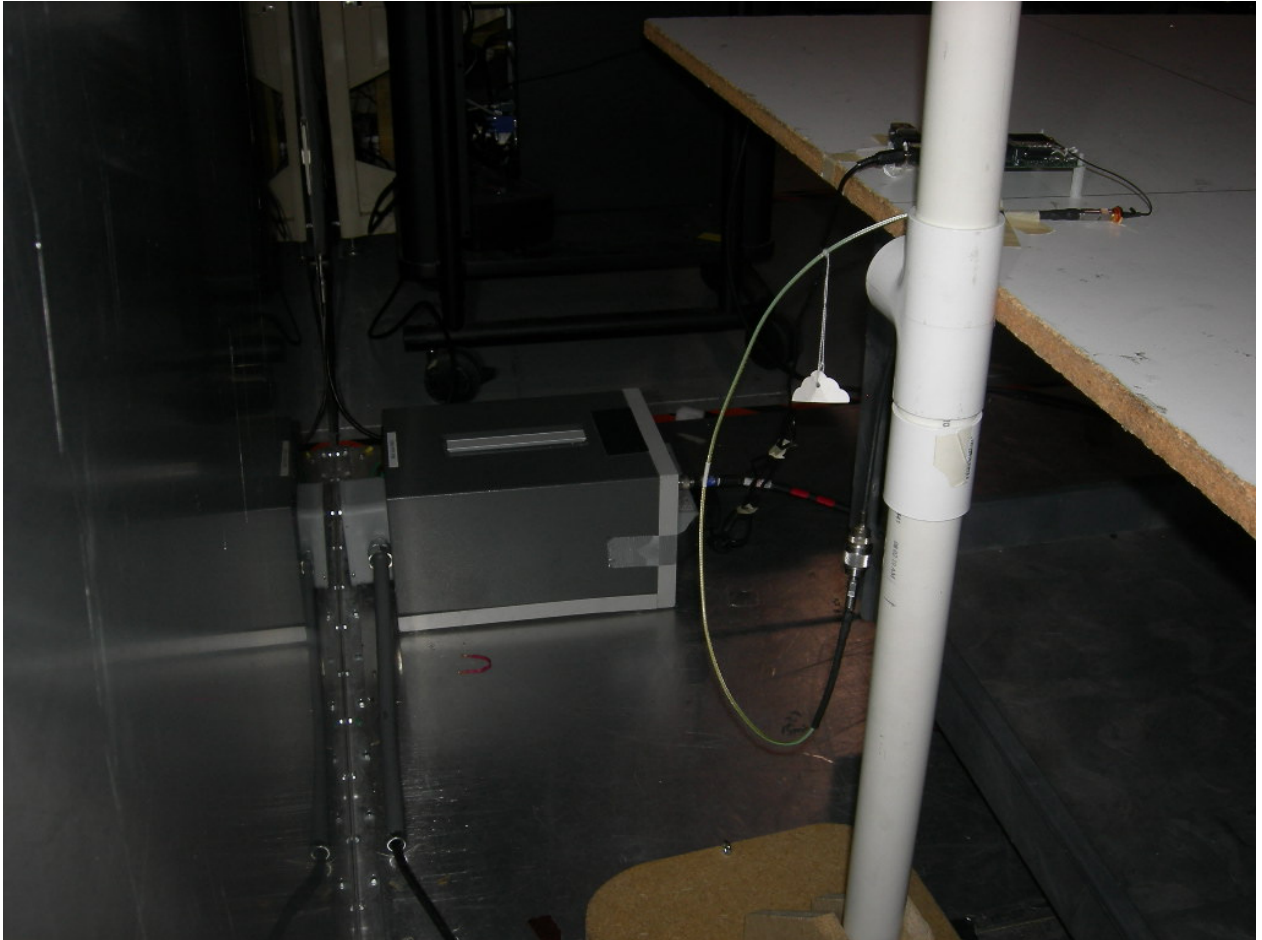
Figure 6: AC Power Line Conducted Emissions – Dipole Antenna
