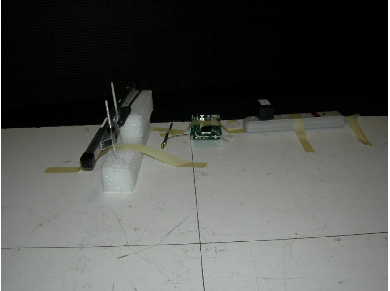
Figure 4: Radiated Emissions – Yagi Antenna
