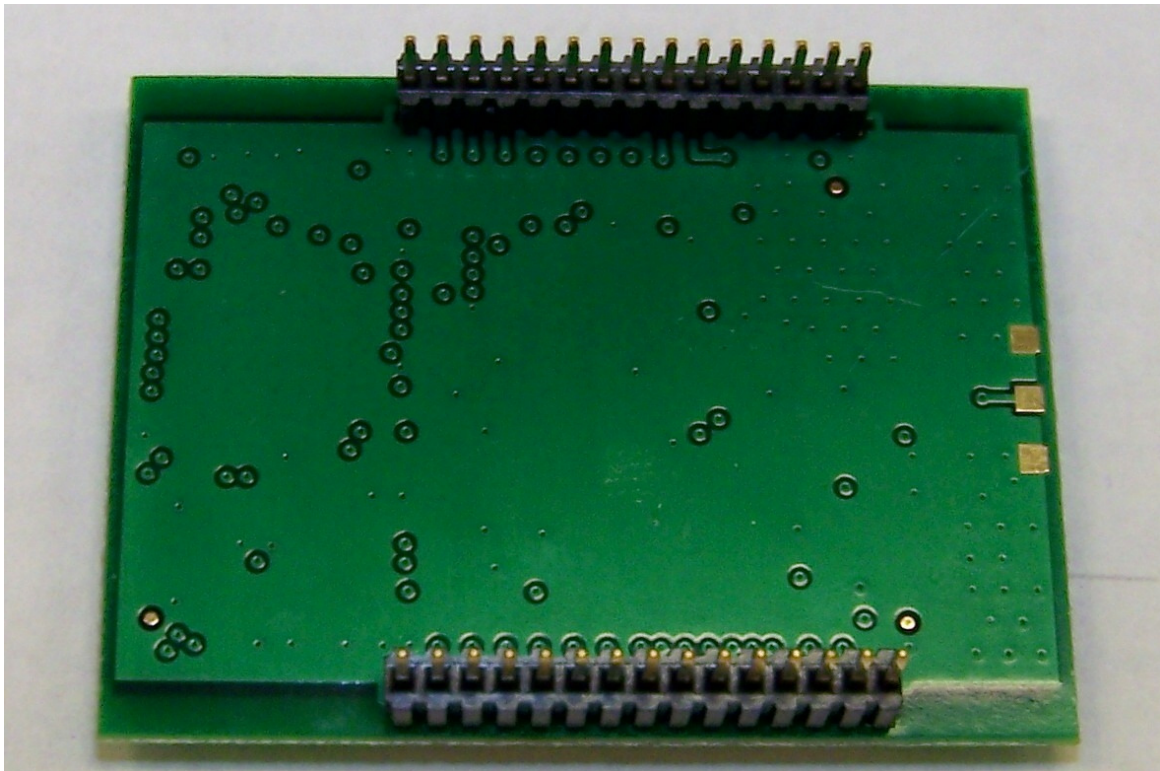
Figure 2: PCB - Back
