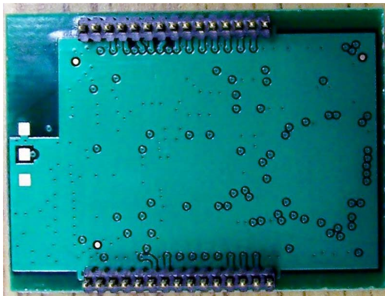
DNT24C and DNT24CA Bottom View
