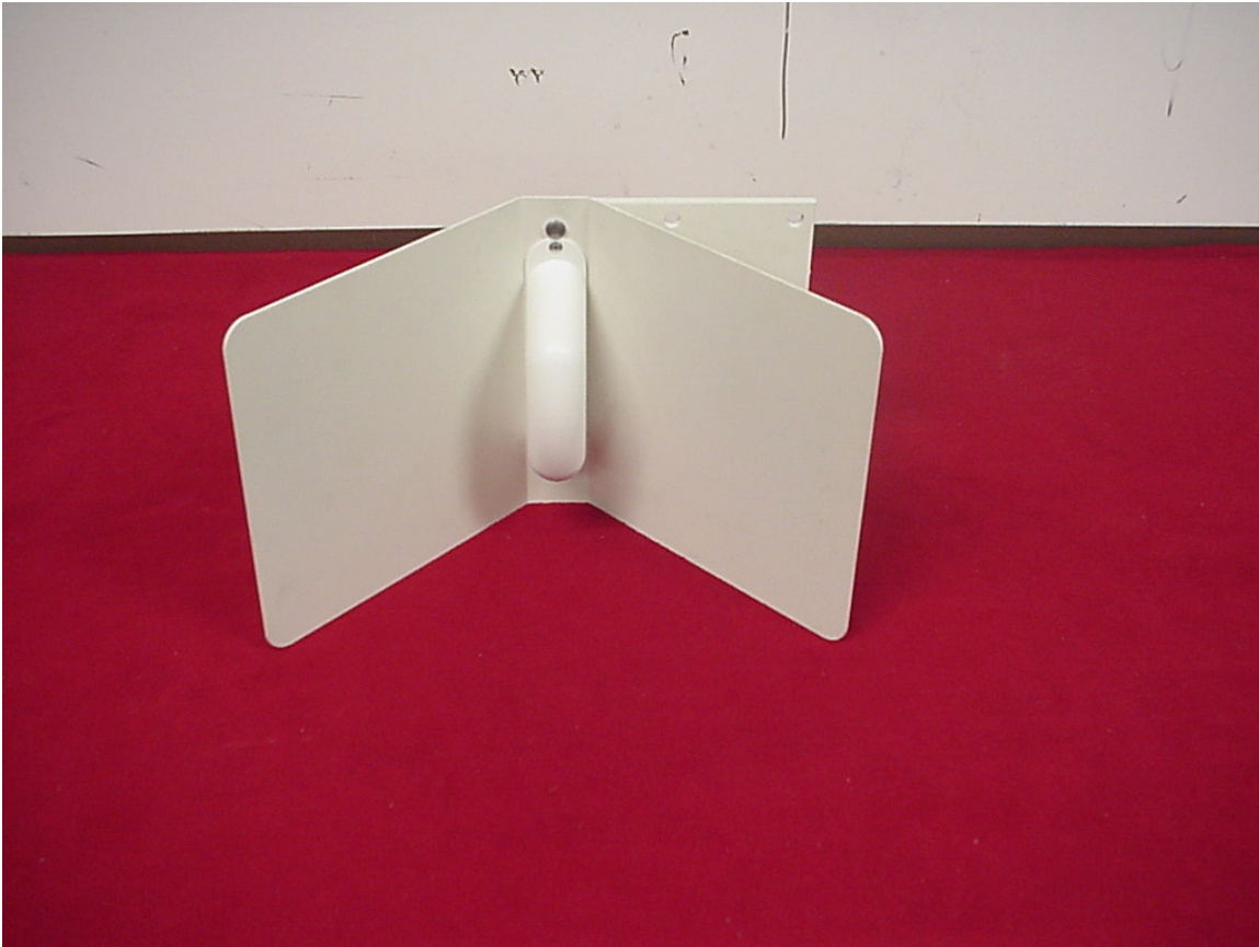
Figure 1. Corner Reflector 14 dBi
