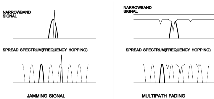
Narrow-band versus spread-spectrum transmission Figure 1.1.1
