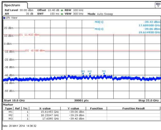
Figure 7.5.1.2-14: 10 GHz – 25 GHz – LCH
