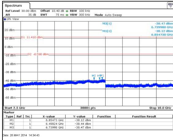
Figure 7.5.1.2-13: 2.5 GHz – 10 GHz – LCH
