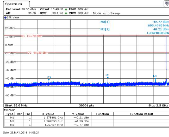
Figure 7.5.1.2-15: 30 MHz – 2.5 GHz – MCH
