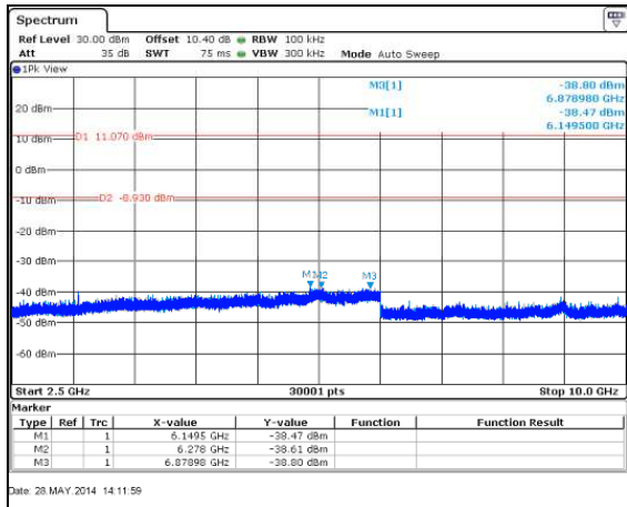
Figure 7.5.1.2-16: 2.5 GHz – 10 GHz – MCH
