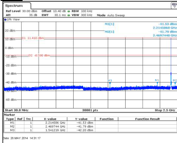
Figure 7.5.1.2-12: 30 MHz – 2.5 GHz – LCH
