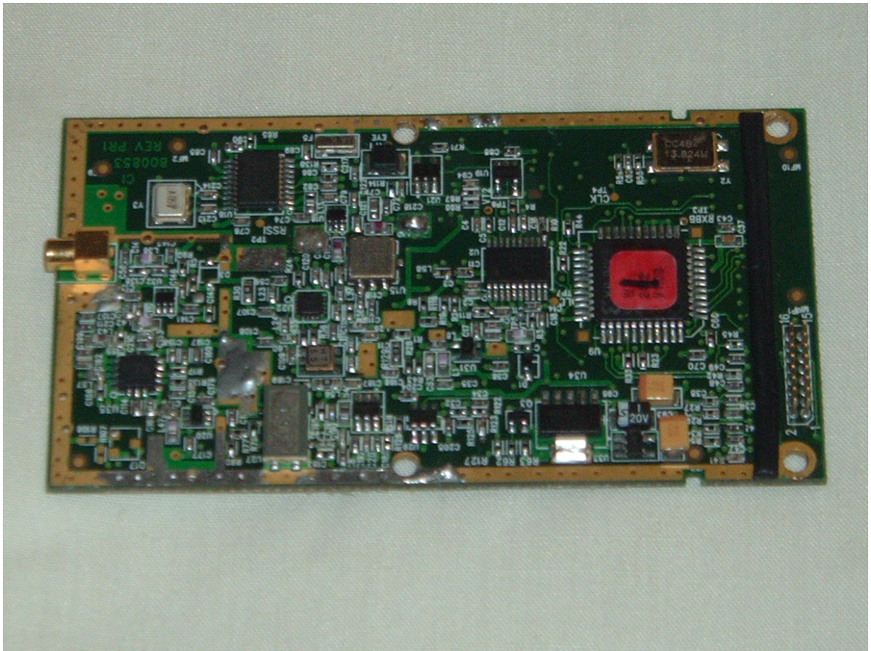
Photo 3 Top View of EUT
