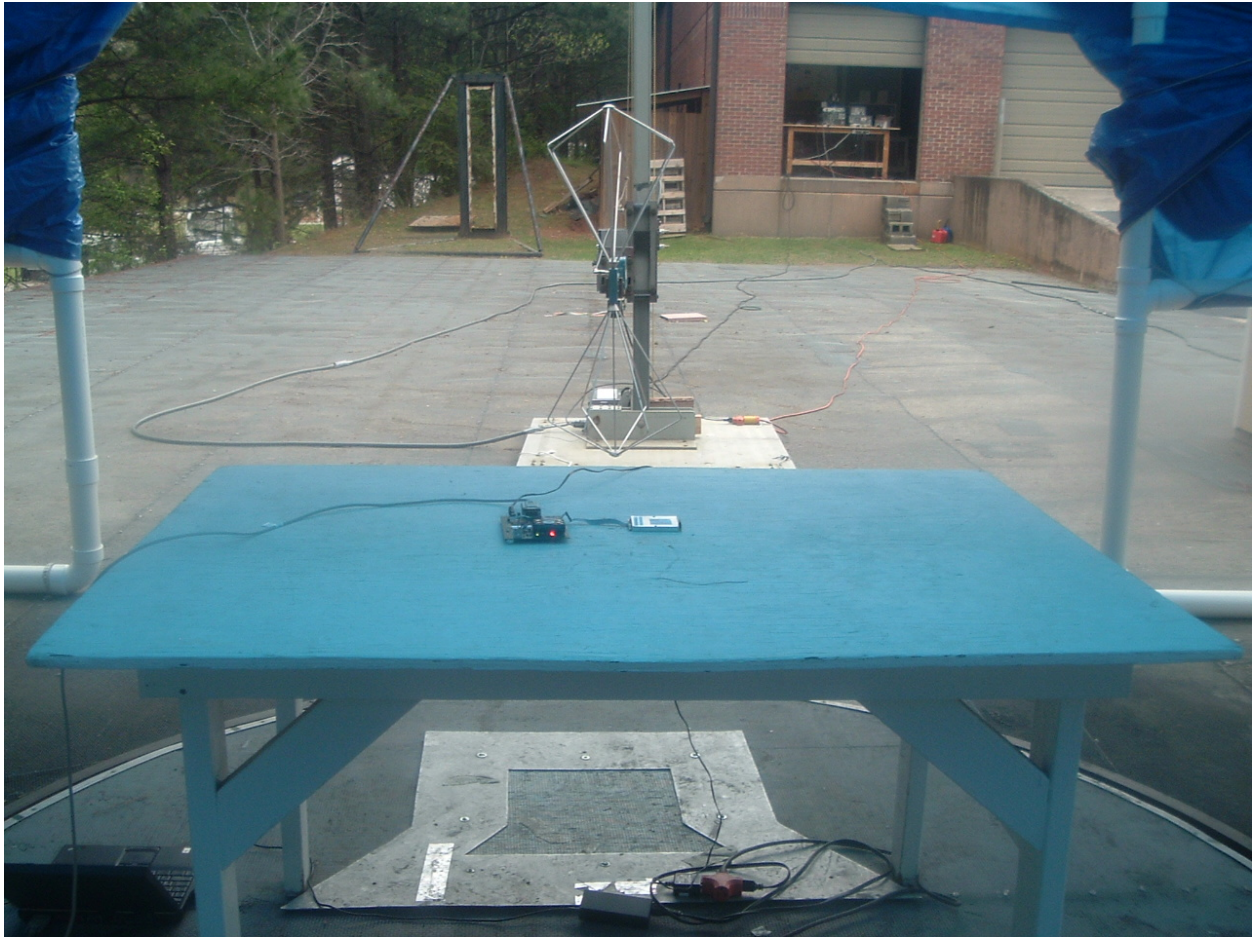
Photo 4. Back View of EUT Patch Antenna
