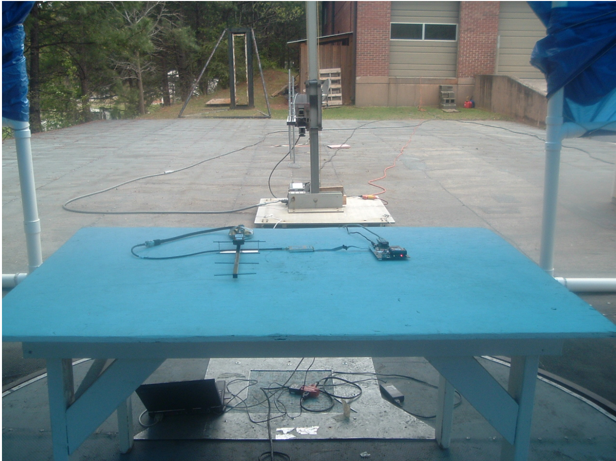
Photo 3. Back View of EUT Yagi Antenna
