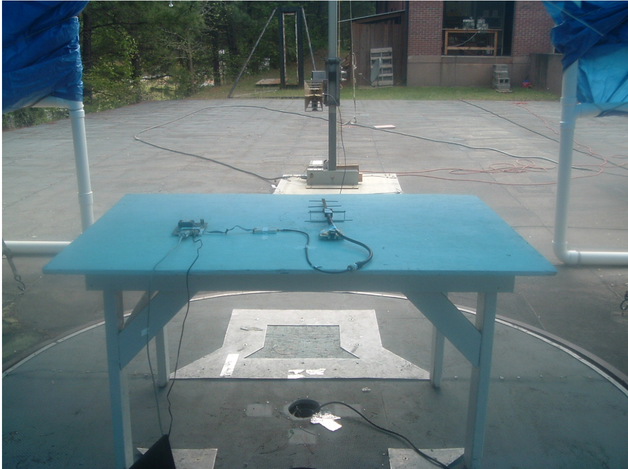
Photo 5. Above 1GHz Test setup at 3 meters
