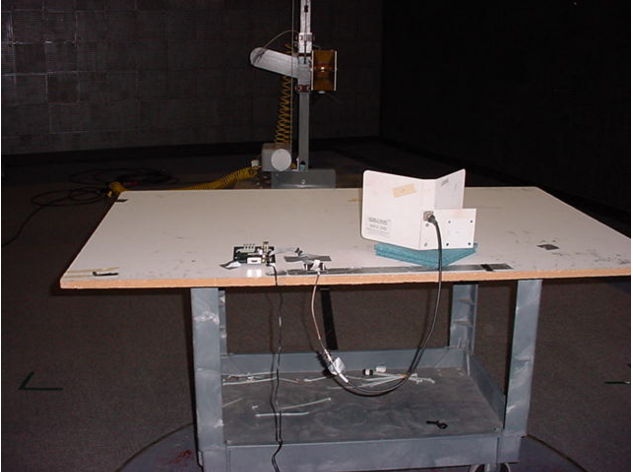
Figure 2: Radiated Emissions - 14dB Corner Reflector
