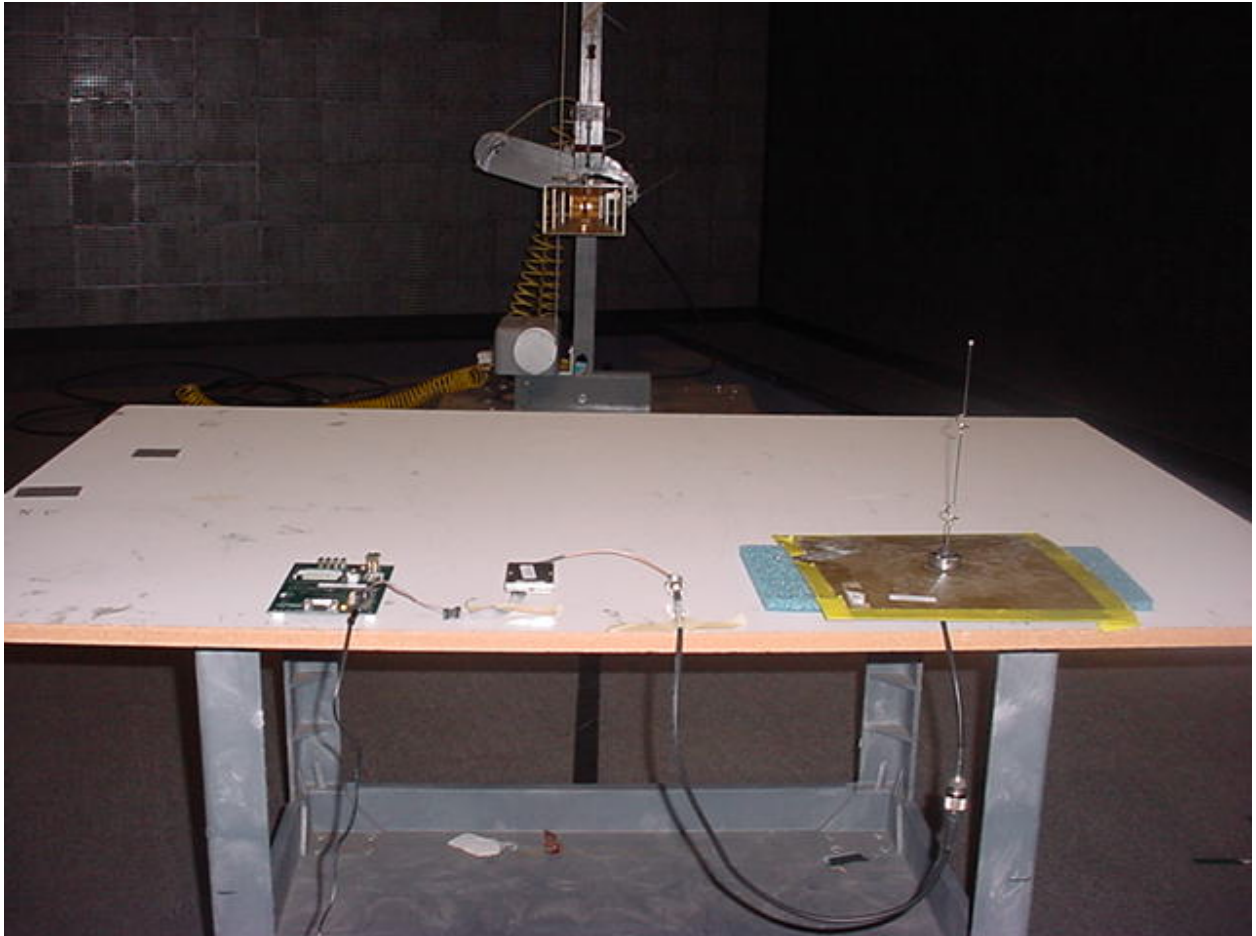
Figure 5: Radiated Emissions - 5dB Mobile Mount
