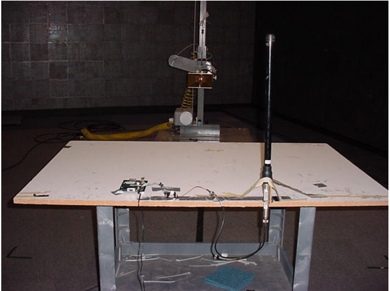
Figure 3: Radiated Emissions - 9dB Omni-directional / Dipole
