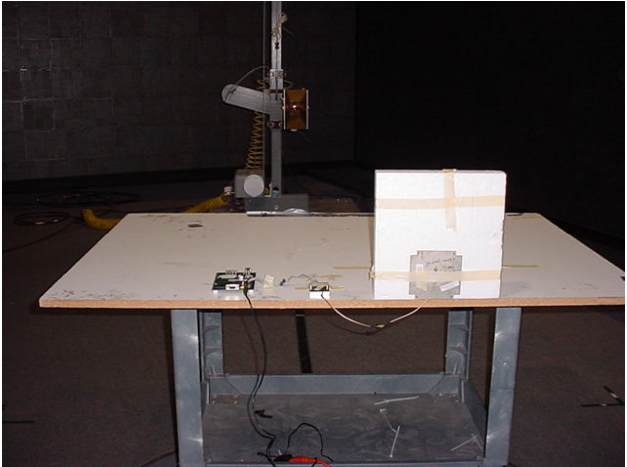
Figure 4: Radiated Emissions - 12dB Cironnet Patch
