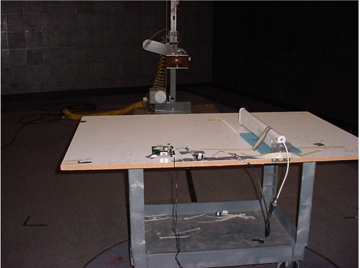
Figure 1: Radiated Emissions - 15dB Yagi Direction Antenna
