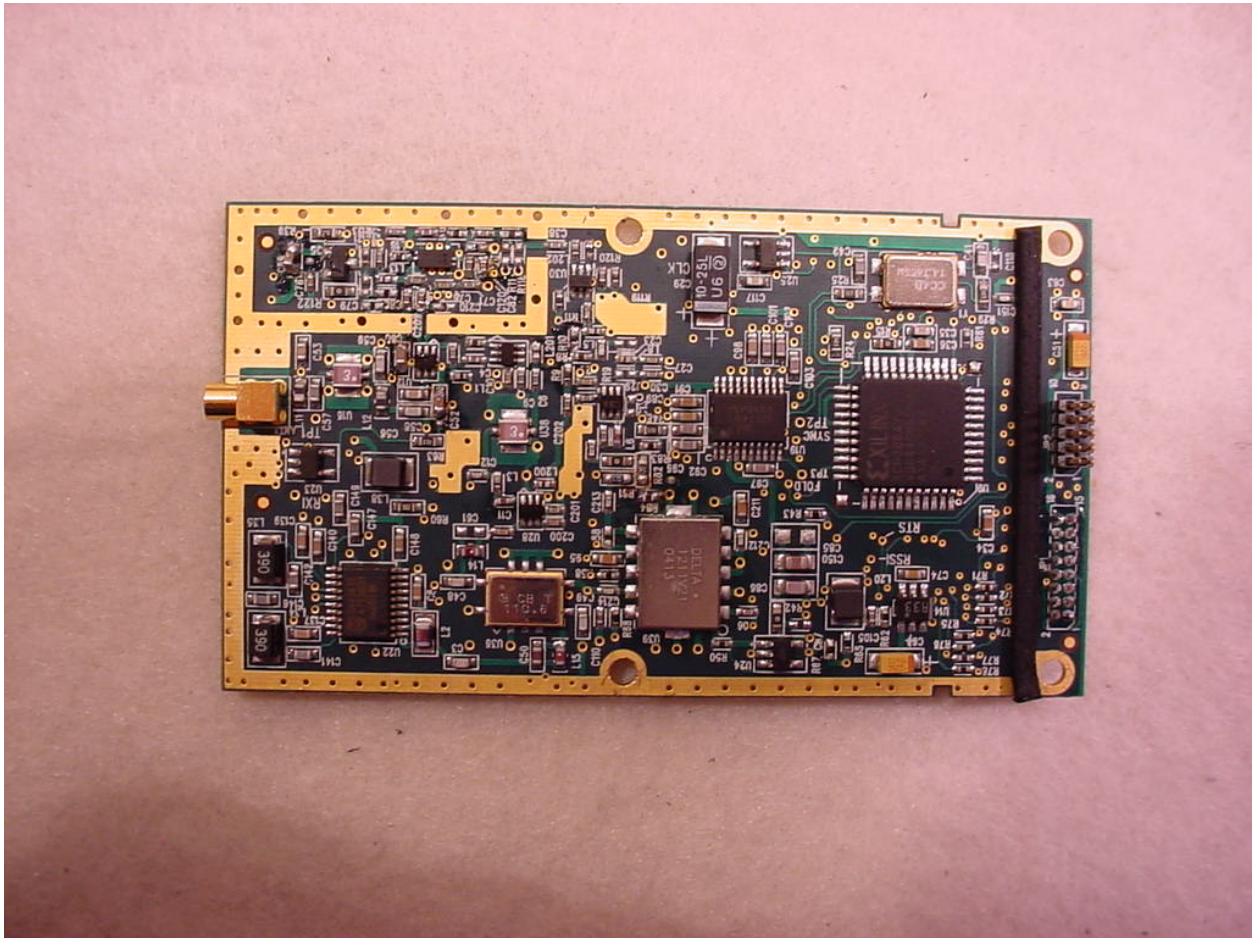
Figure 1: Internal Photographs – PCB Top
