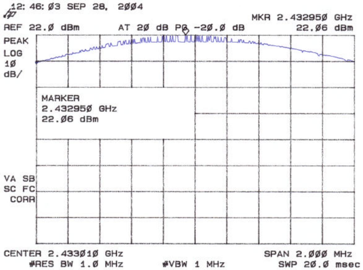
Figure 3b. Peak Power per FCC Section 15.247( b) Low Mid Channel
