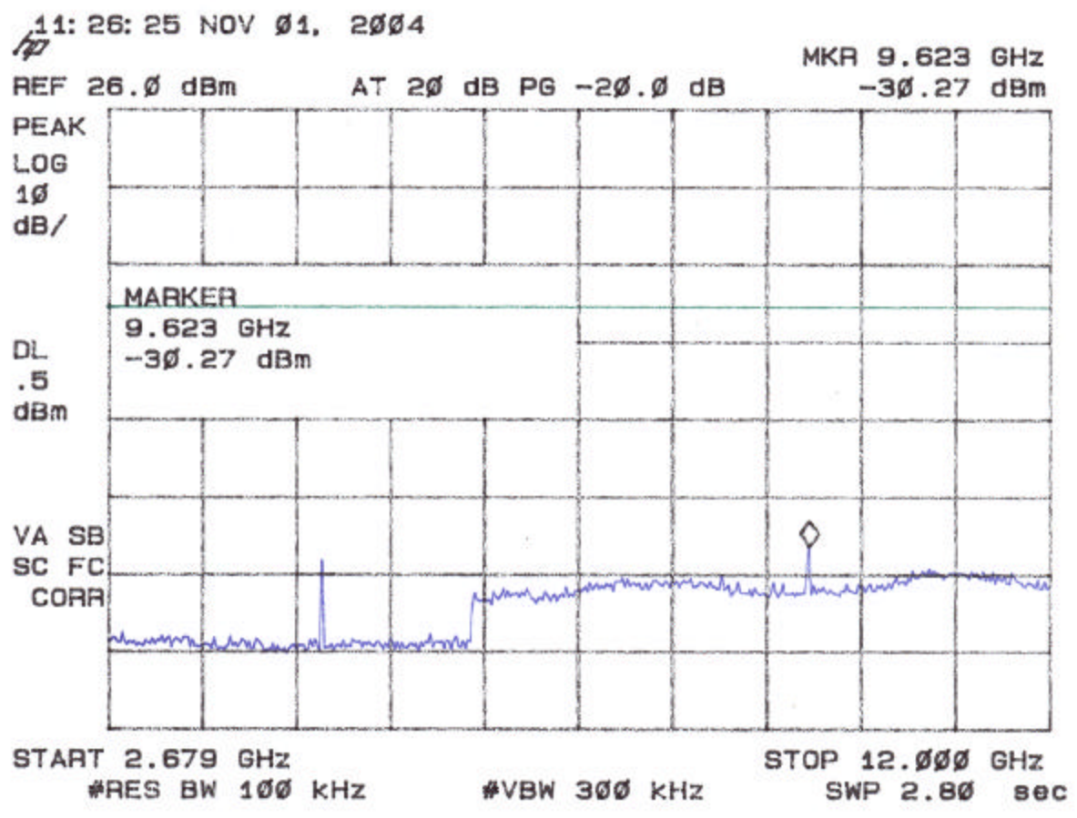
Figure 4c Antenna Conducted Spurious Emissions 15.247(c) Low
