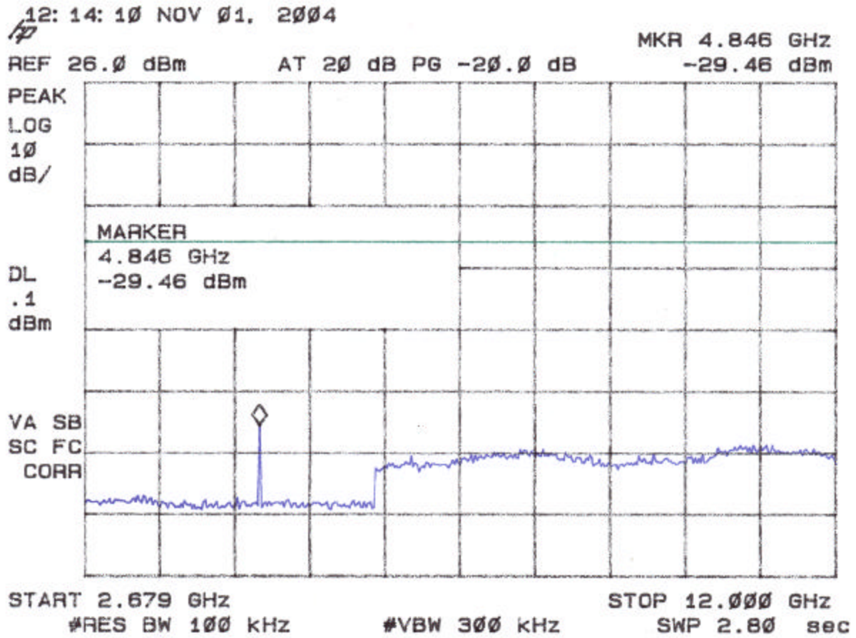
Figure 4g Antenna Conducted Spurious Emissions 15.247(c) Low Mid
