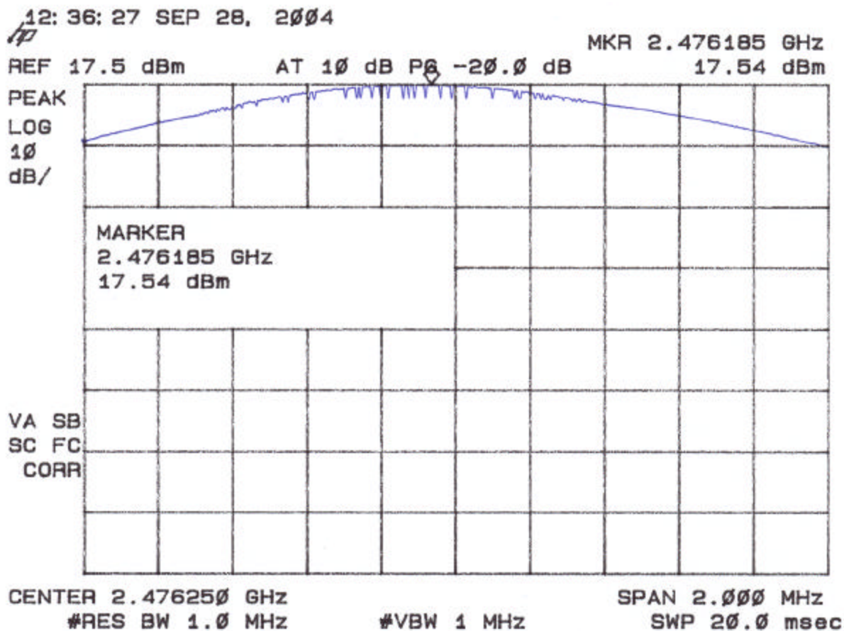
Figure 3d. Peak Power per FCC Section 15.247( b) (High Channel)
