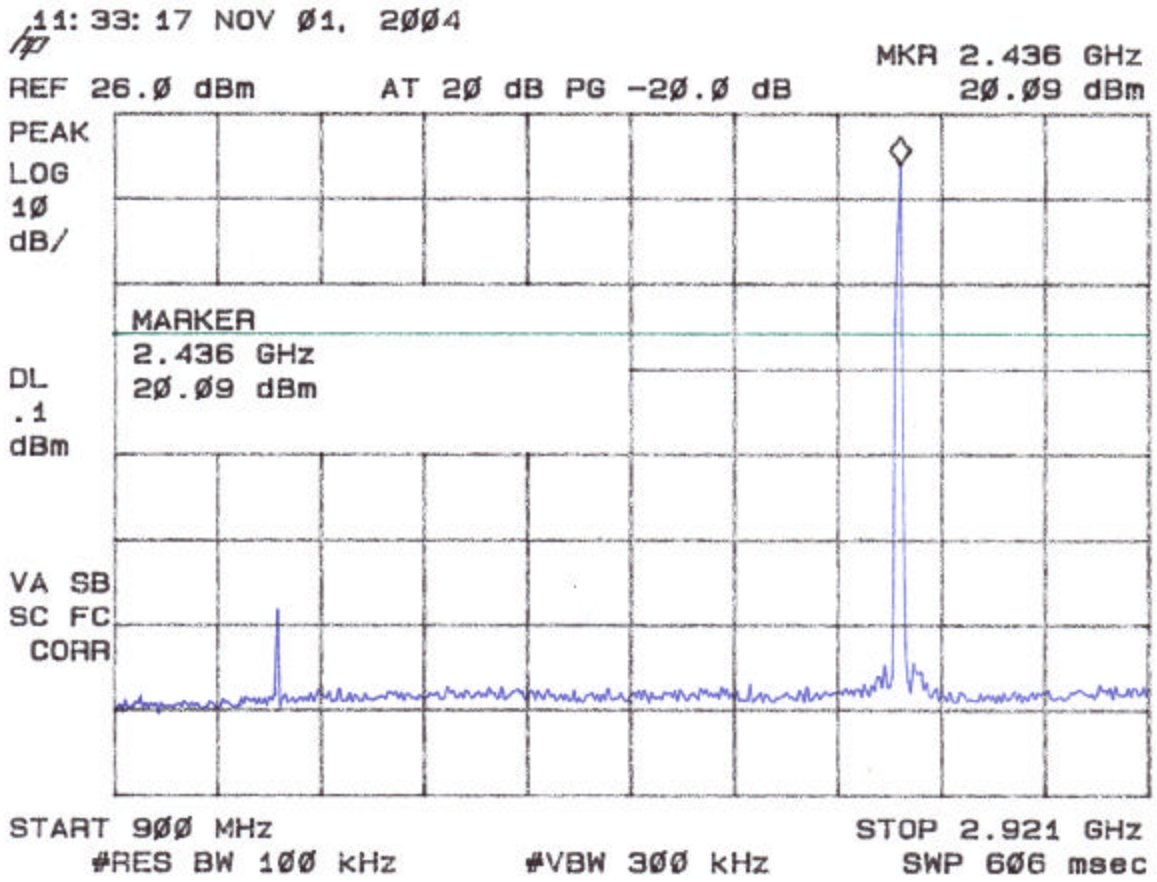
Figure 4f Antenna Conducted Spurious Emissions 15.247(c) Low Mid
