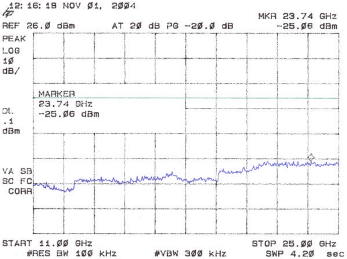
Figure 4h Antenna Conducted Spurious Emissions 15.247(c) Low Mid
