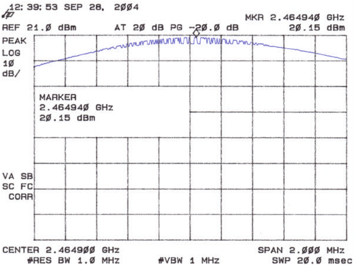
Figure 3c. Peak Power per FCC Section 15.247( b) (High Mid Channel)
