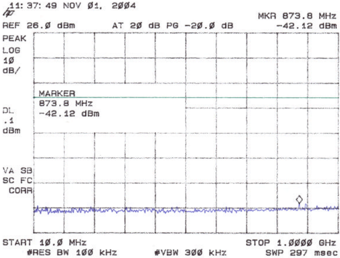
Figure 4e Antenna Conducted Spurious Emissions 15.247(c) Low Mid
