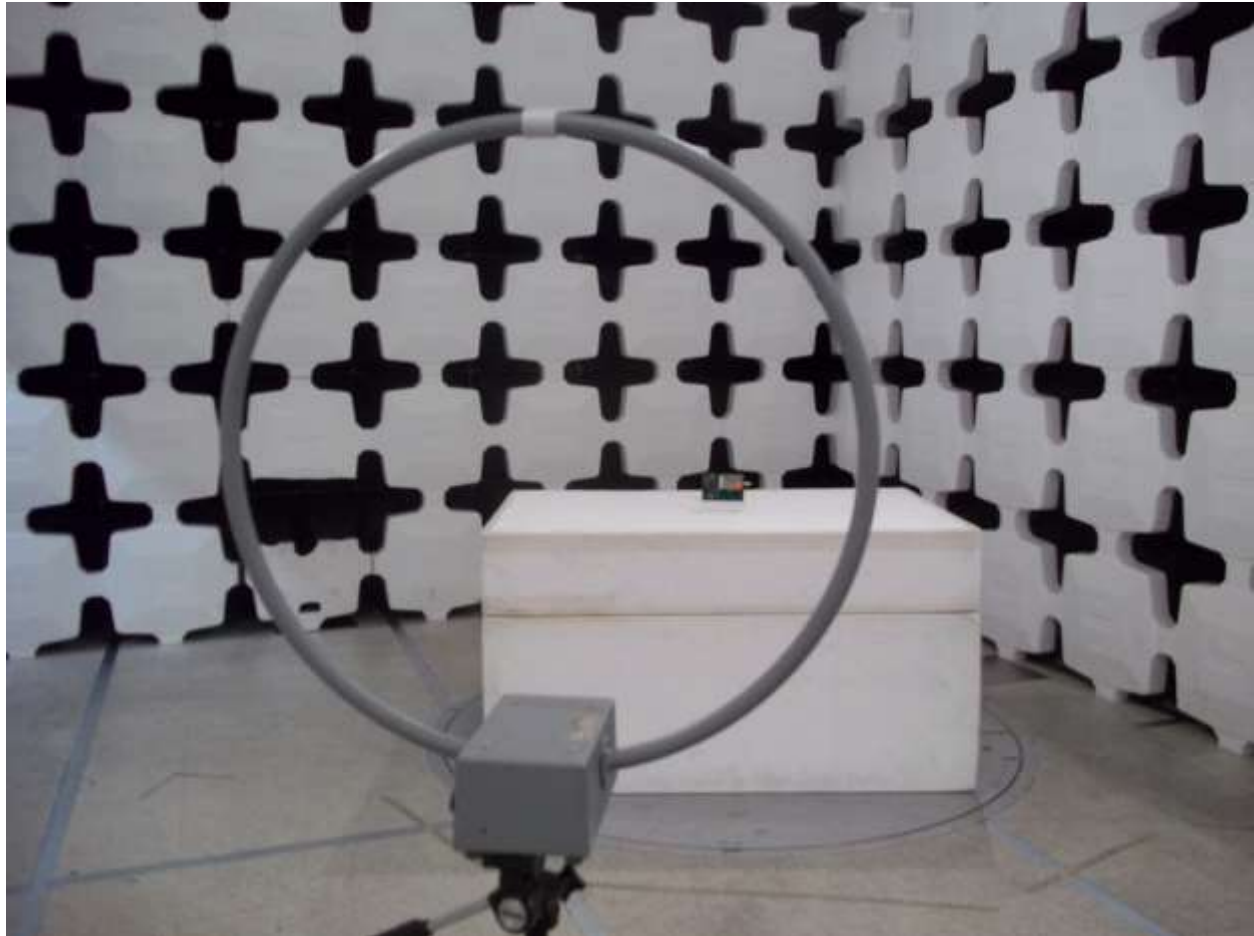
Figure 8. Radiated Spurious Emissions: 9 kHz to 30 MHz
