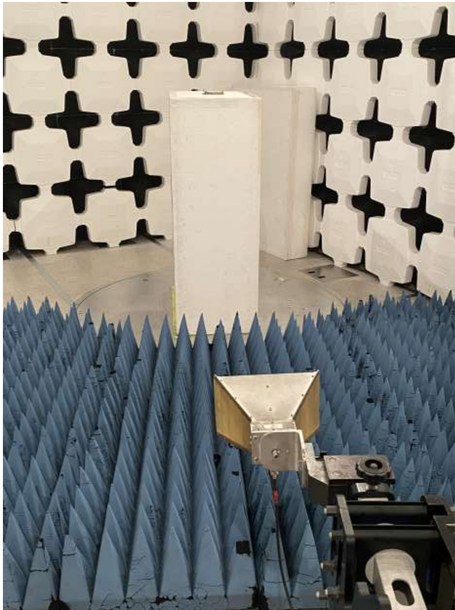
Figure 6. Radiated Emissions, 1 GHz to 25 GHz Test Setup: EUT with Patch Antenna
