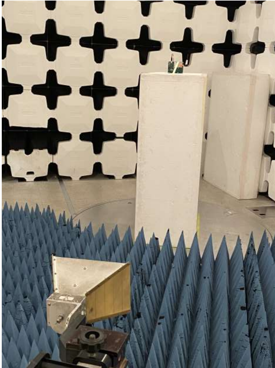
Figure 4. Radiated Emissions, 1 GHz to 25 GHz Test Setup: EUT with Dipole Antenna
