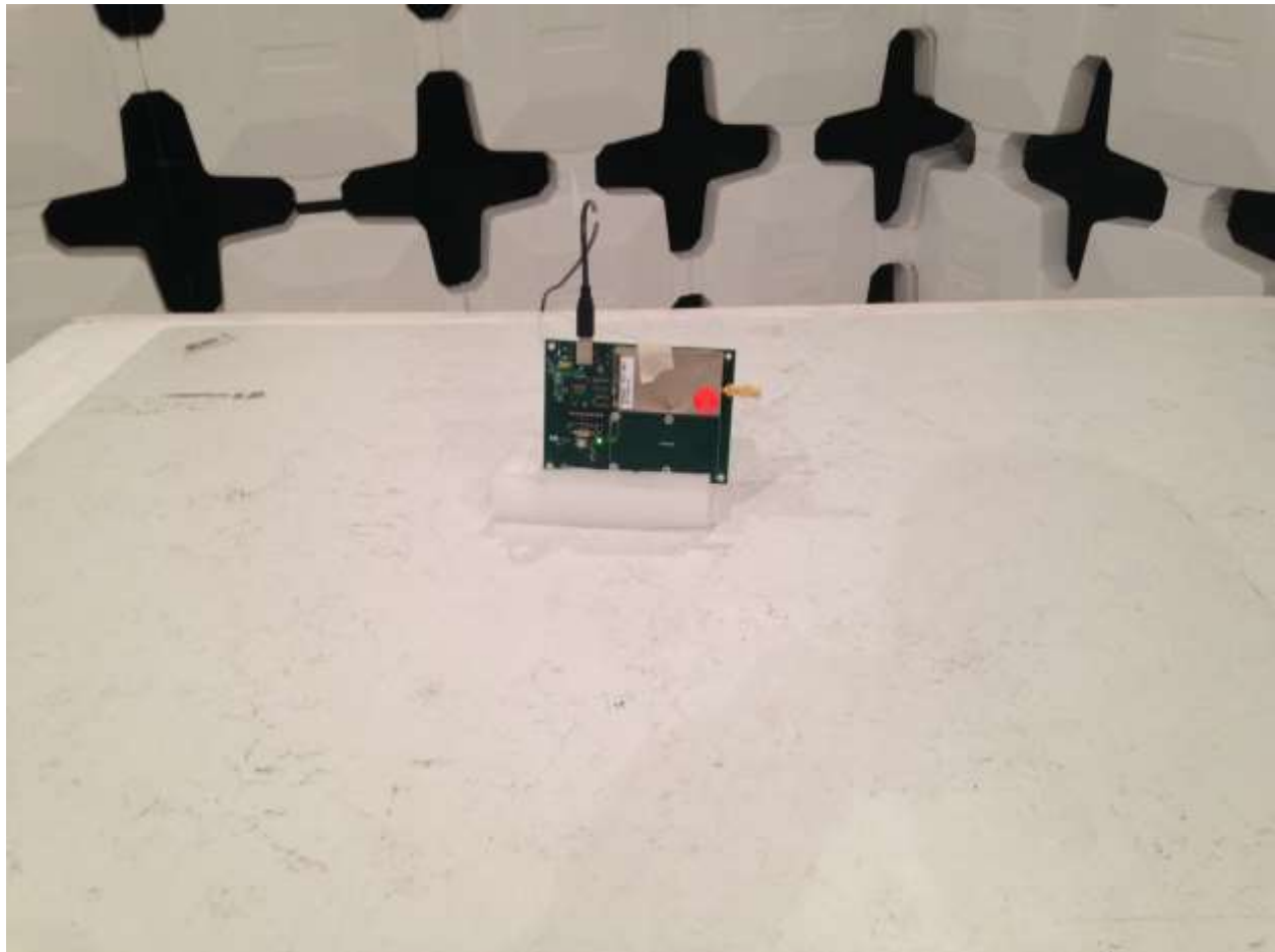
Figure 7. Radiated Spurious Emissions: EUT Worst Case Position Test Setup
