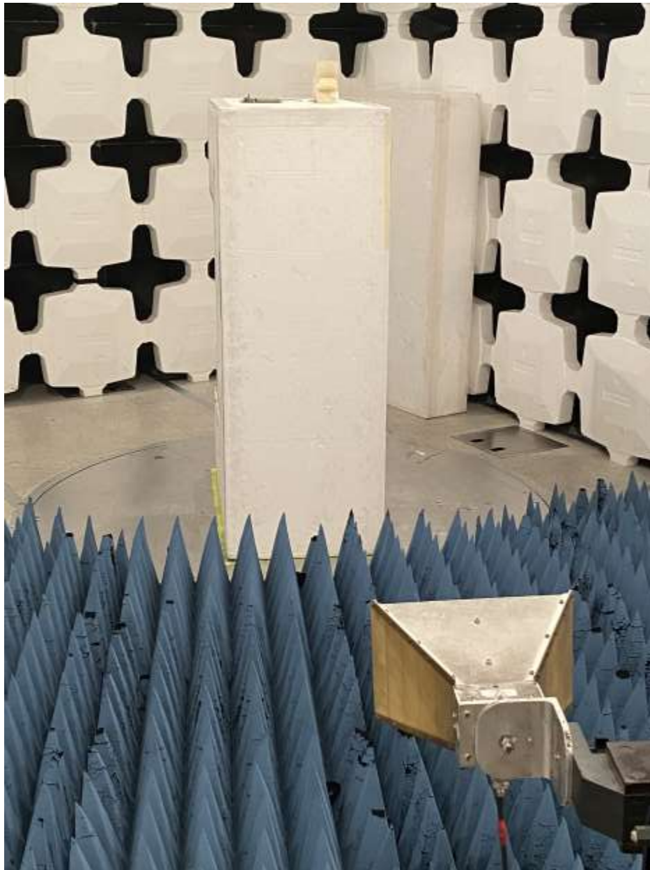
Figure 2. . Radiated Emissions, 1 GHz to 25 GHz Test Setup: EUT with Corner Reflector Antenna
