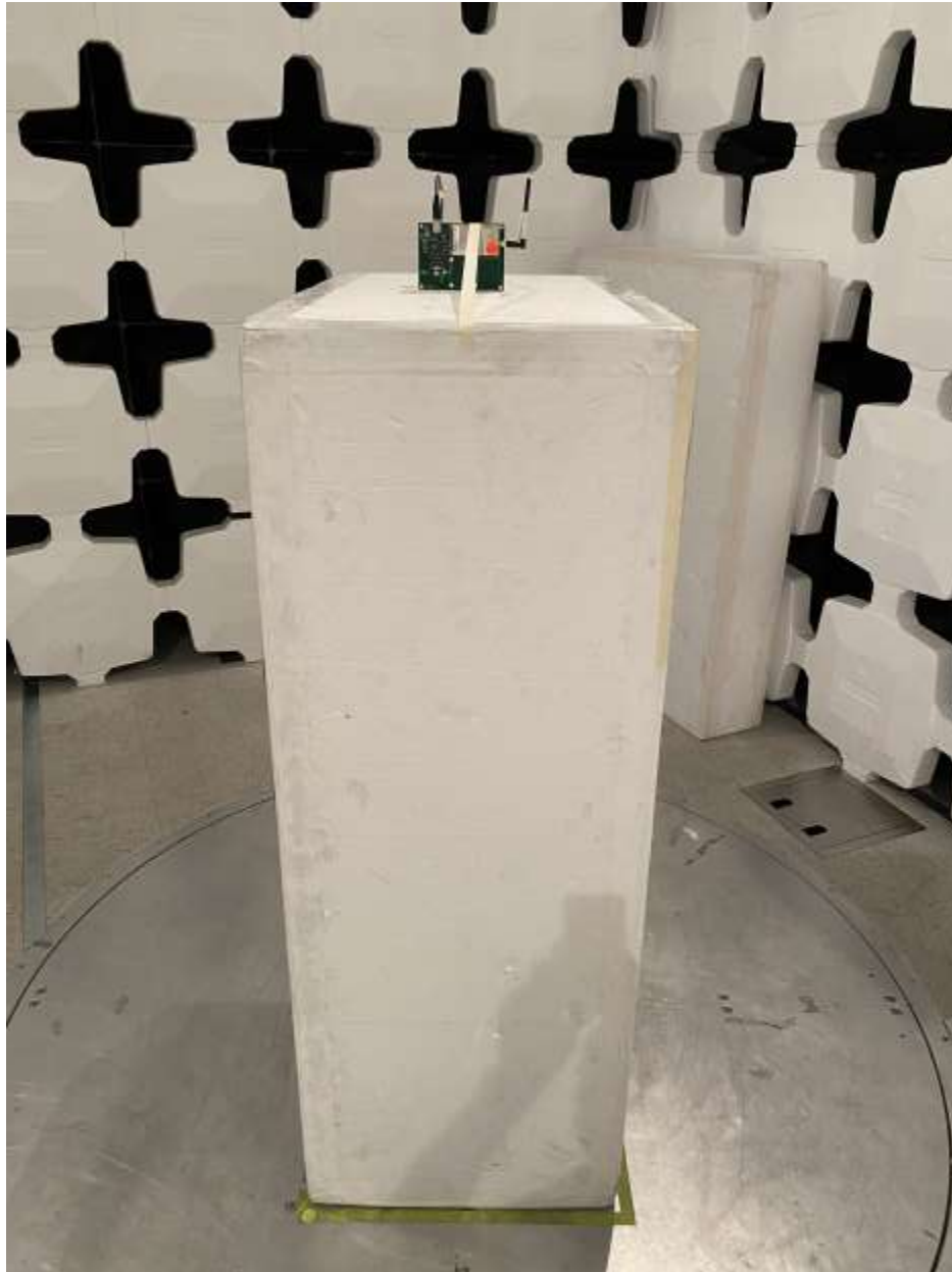
Figure 3. Radiated Emissions, EUT Worst Case Position Test Setup: EUT with Dipole Antenna
