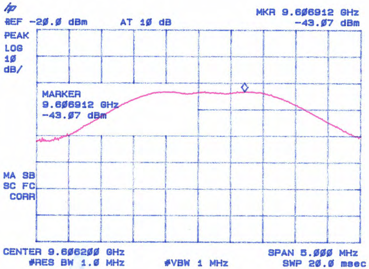
Figure 4a - 4 Peak Radiated Spurious Emission 15.247(c) Low
