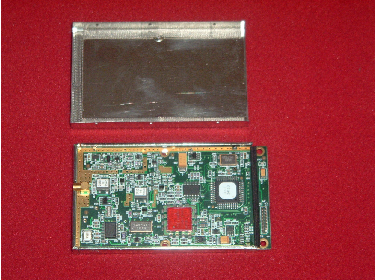
Photo 4. Top of EUT, Cover Open
