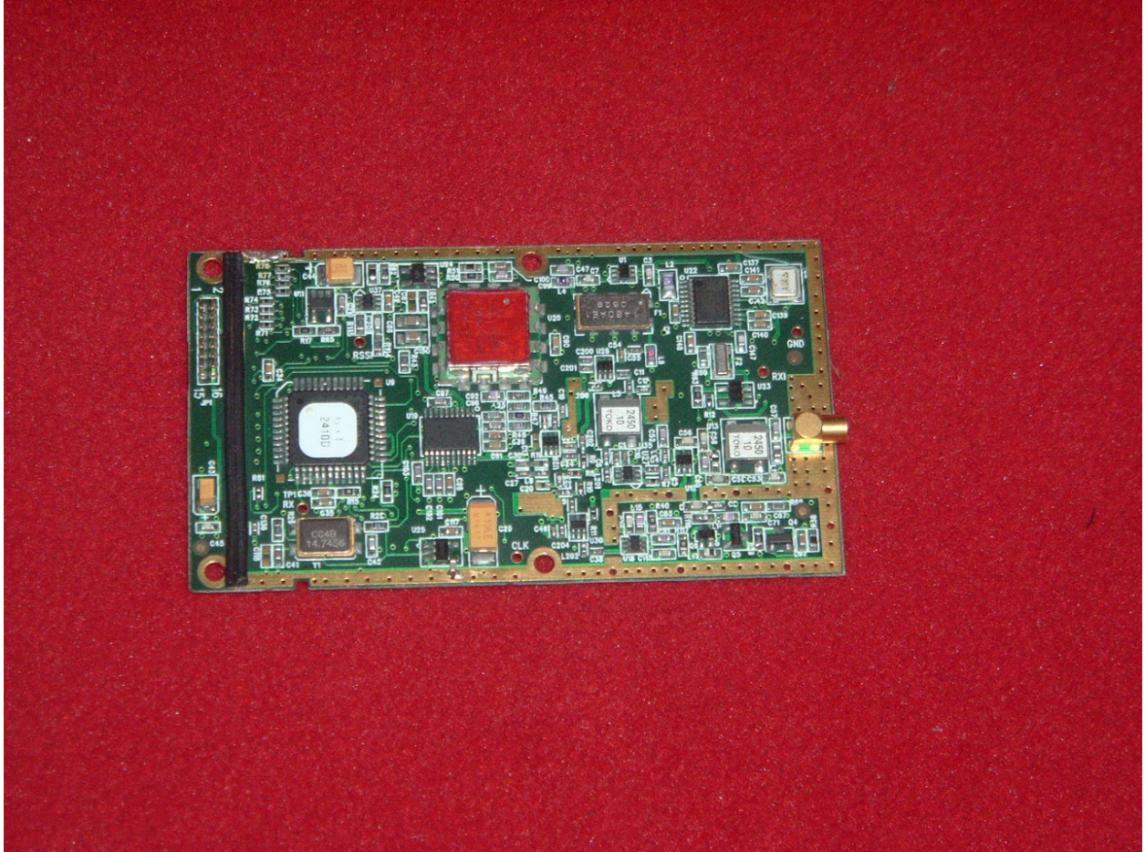
Photo 5. Top of EUT, Cover Removed
