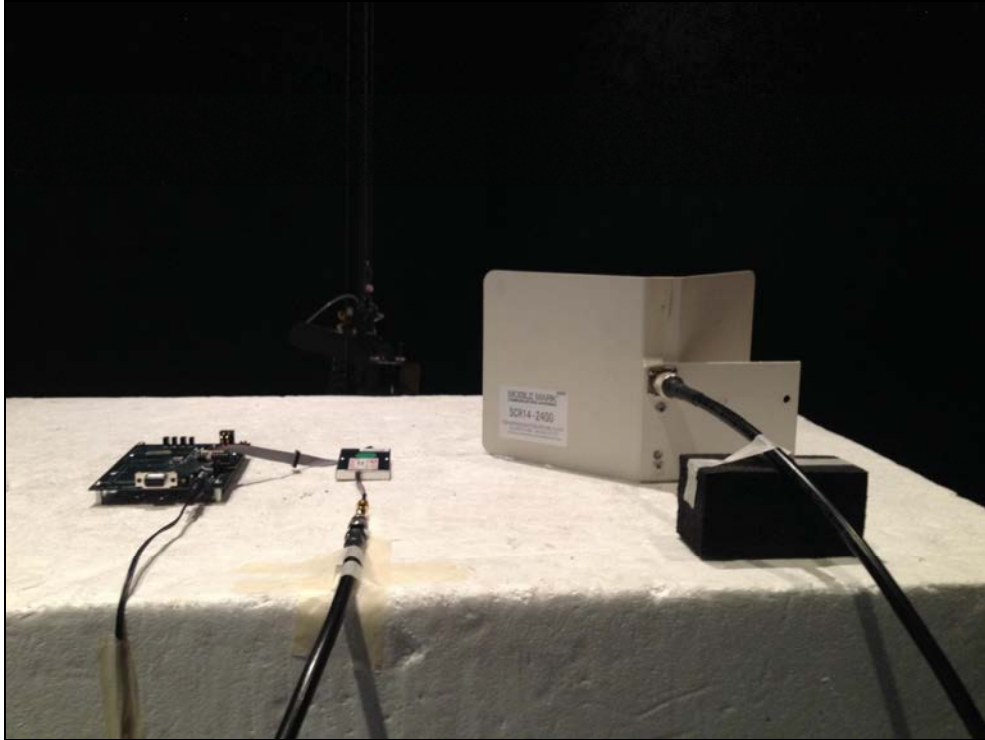
Figure 2: Radiated Emissions – Corner Antenna ZPOS
