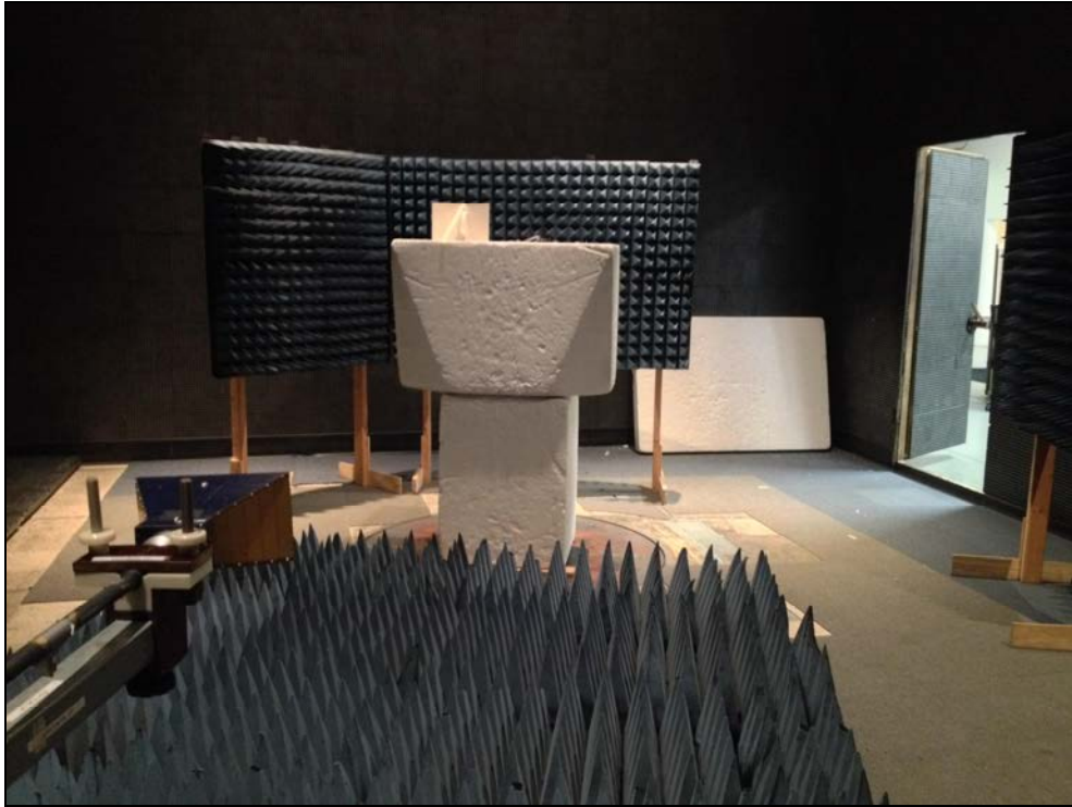
Figure 1: Radiated Emissions – Corner Antenna ZPOS
