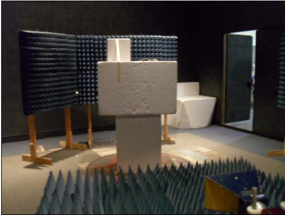
Figure 5: Radiated Emissions – Panel Antenna ZPOS
