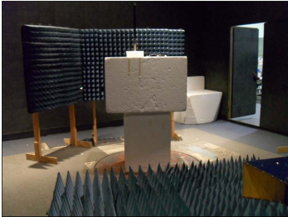
Figure 3: Radiated Emissions – Dipole Antenna ZPOS
