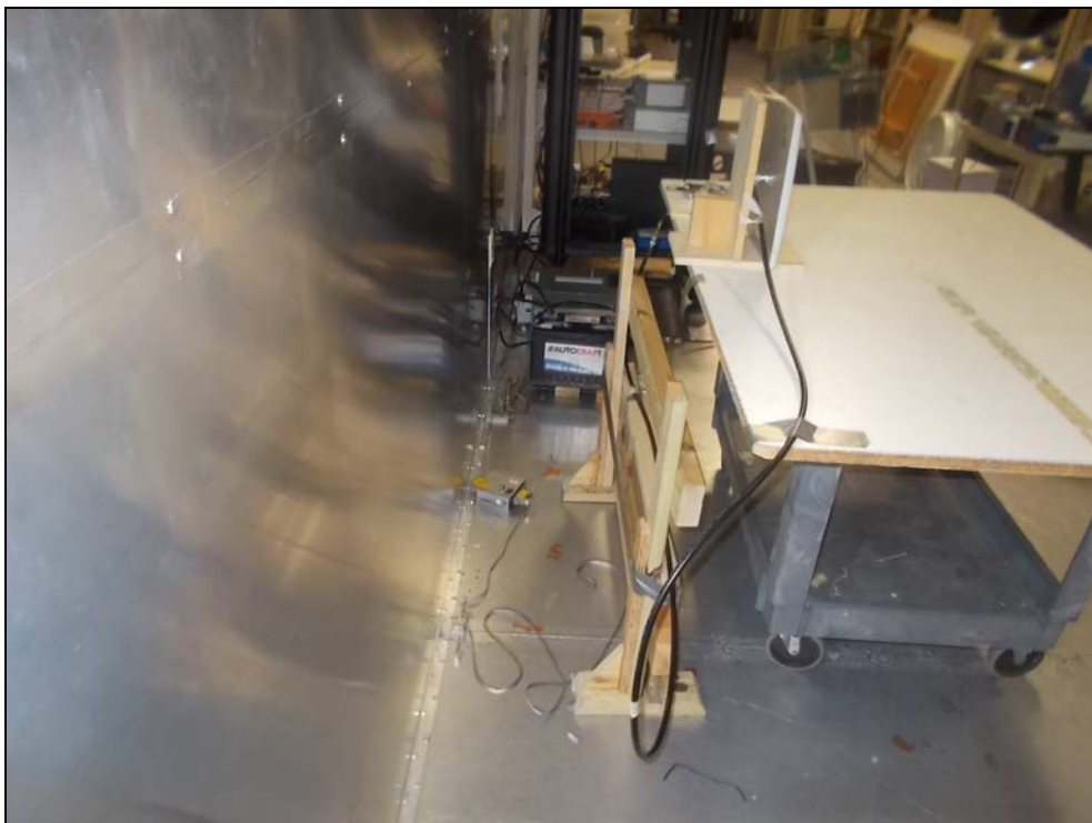
Figure 12: Conducted Emissions – Panel Antenna
