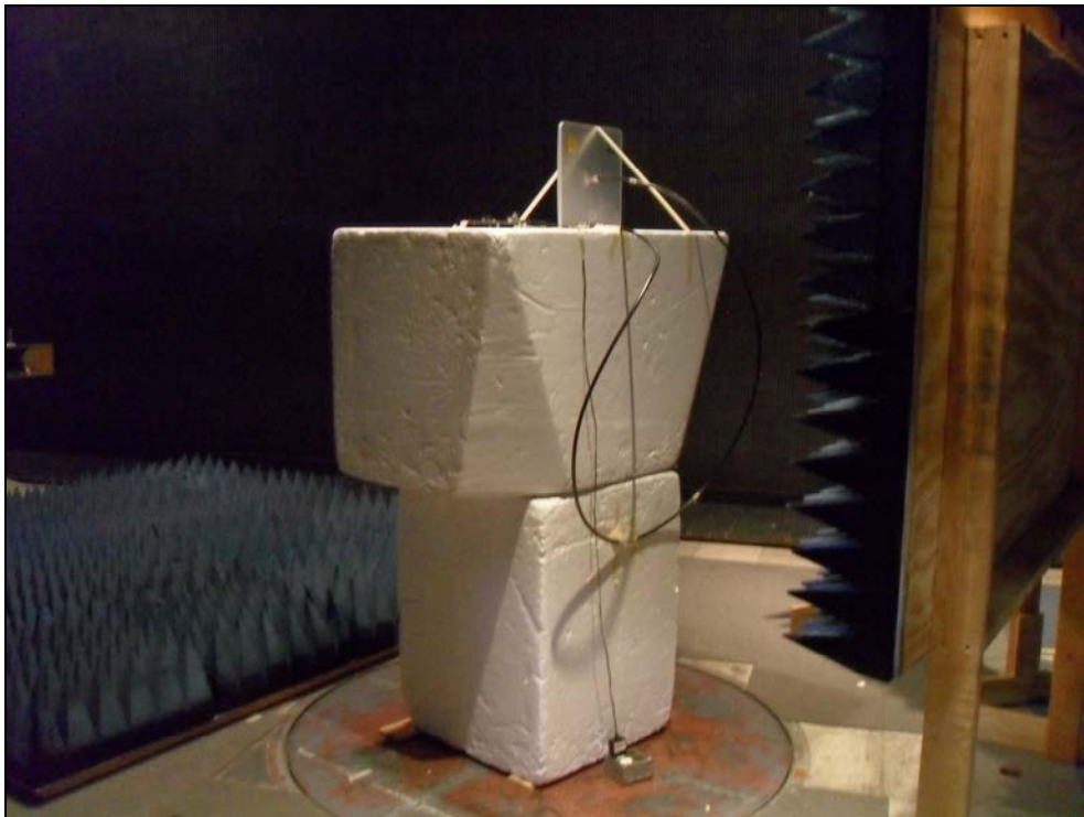
Figure 6: Radiated Emissions – Panel Antenna ZPOS
