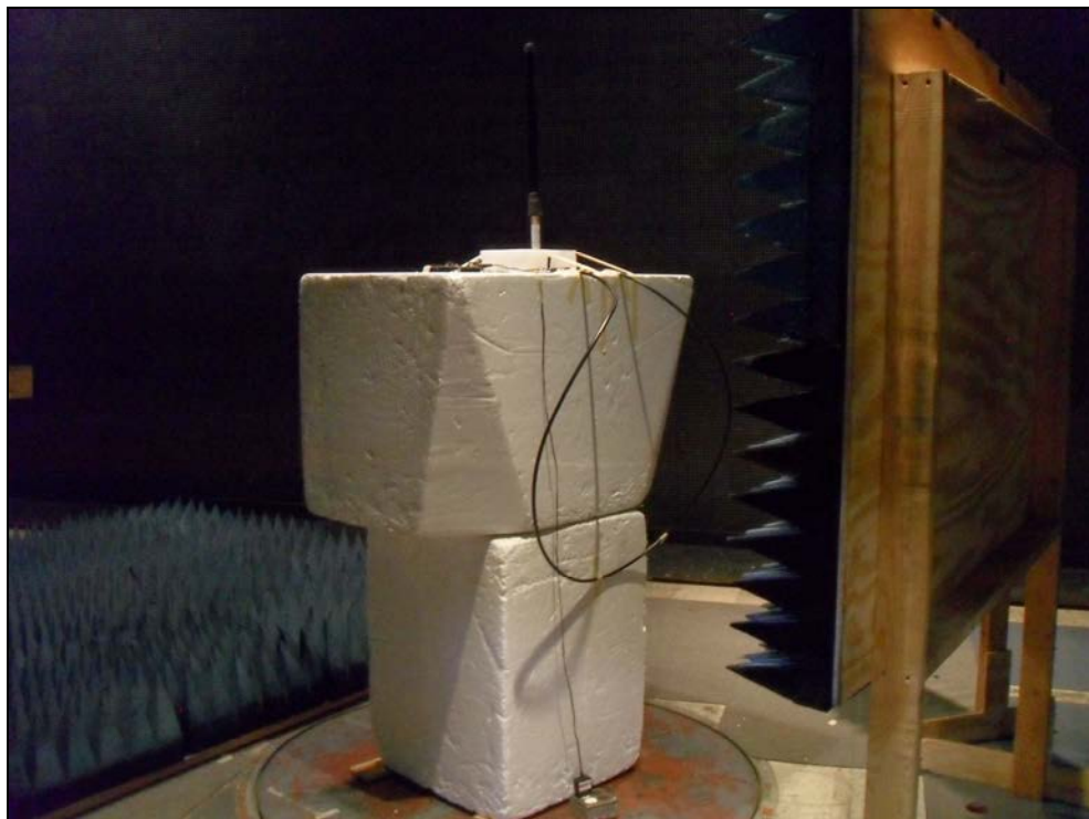
Figure 4: Radiated Emissions – Dipole Antenna ZPOS
