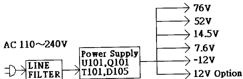
X-770 BLOCK DIAGRAM
