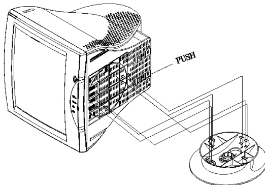
Figure 2 installing the Swivel Base
