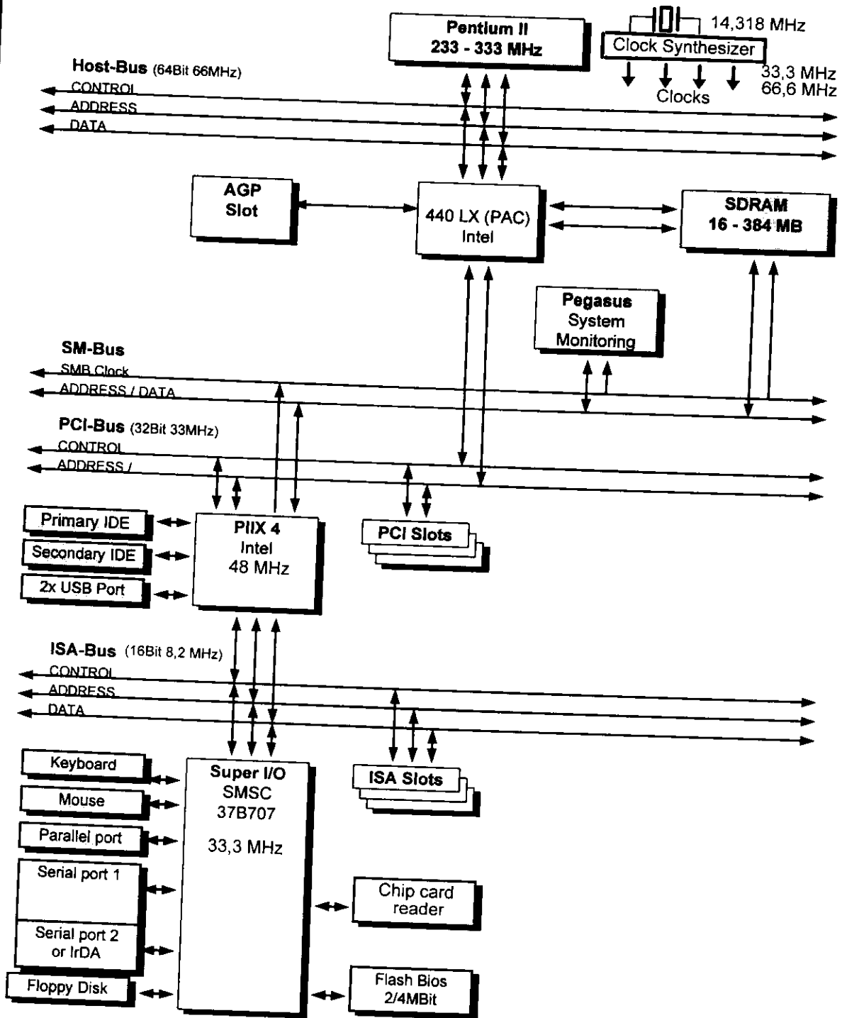
Figure 4.1 Block Diagram of the EUT
