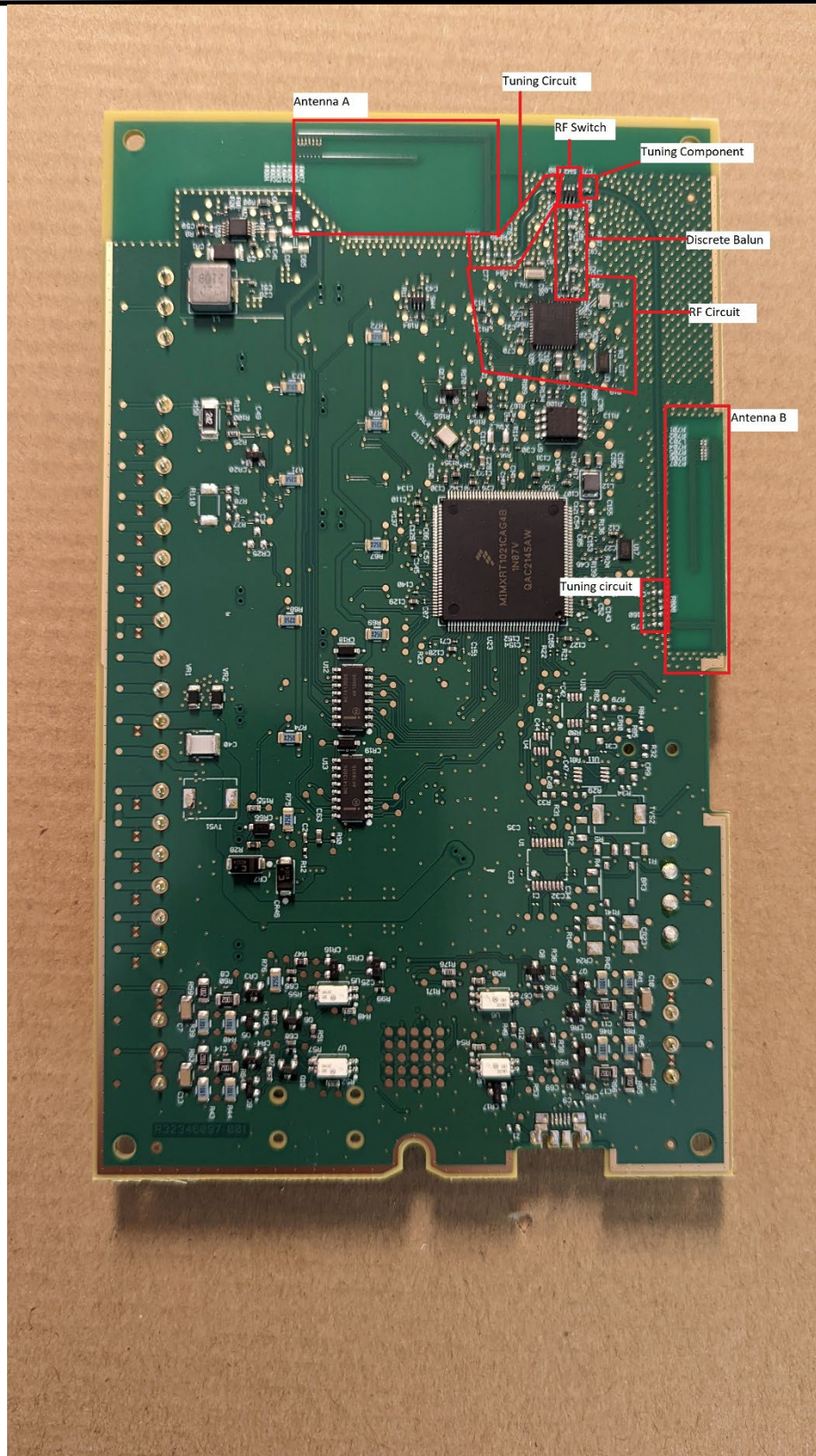
Figure 4. RF circuit identification.
