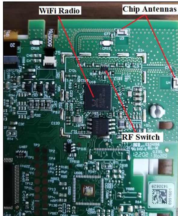
Figure 4. WiFi radio.
