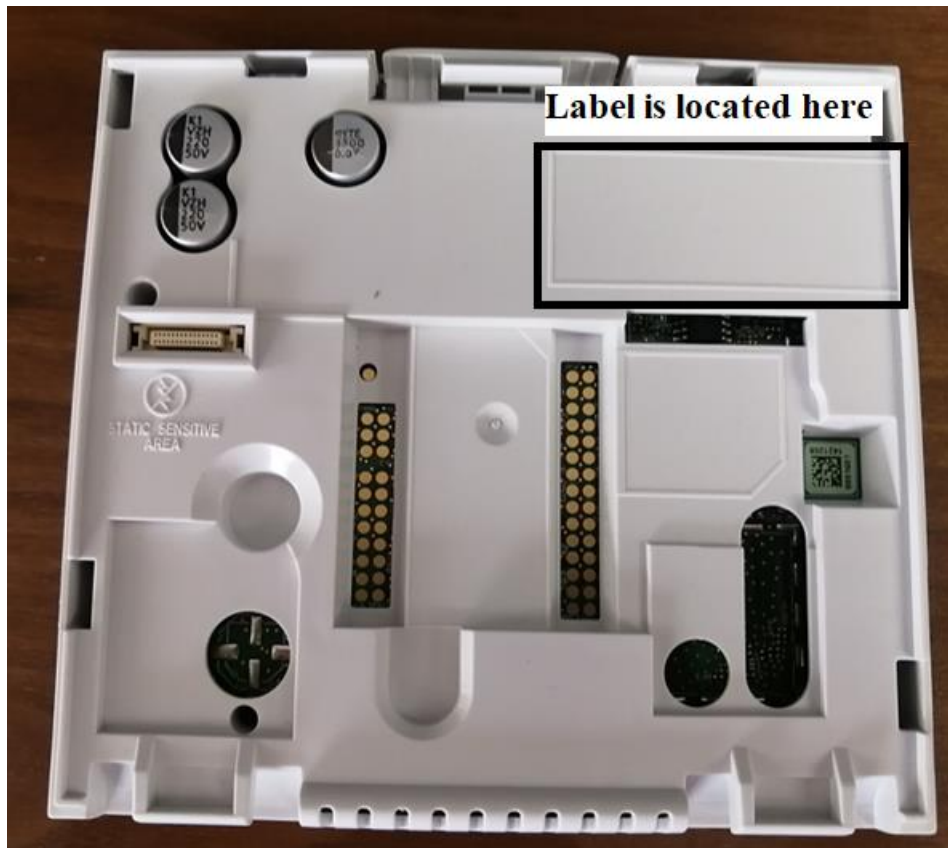
Figure 1. Back side of thermostat – FCC/ISED Label location.
