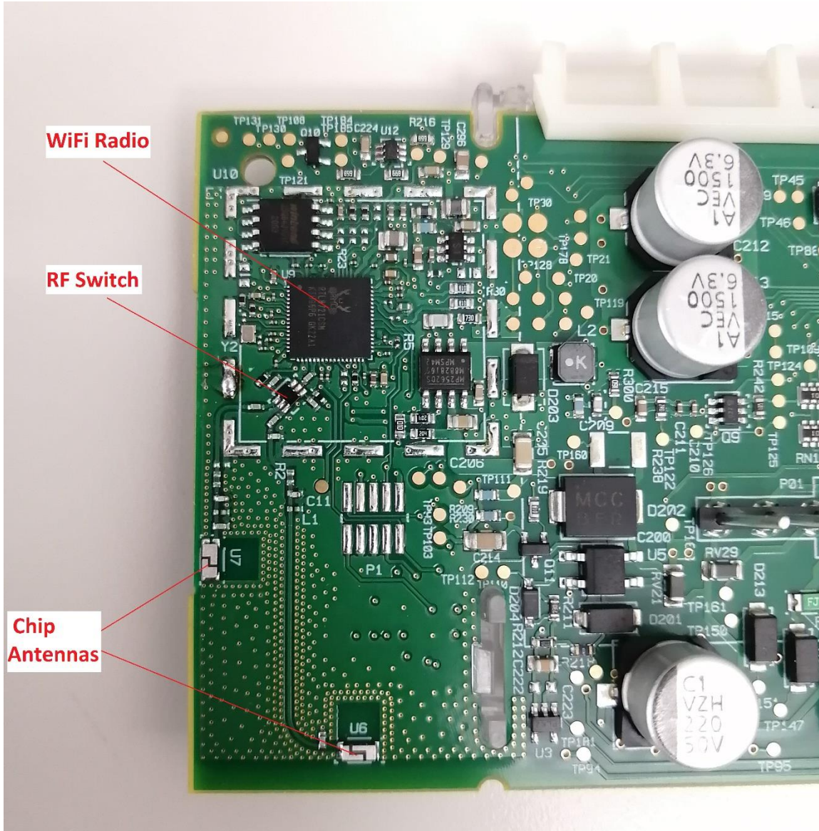
Figure 4. WiFi radio.
