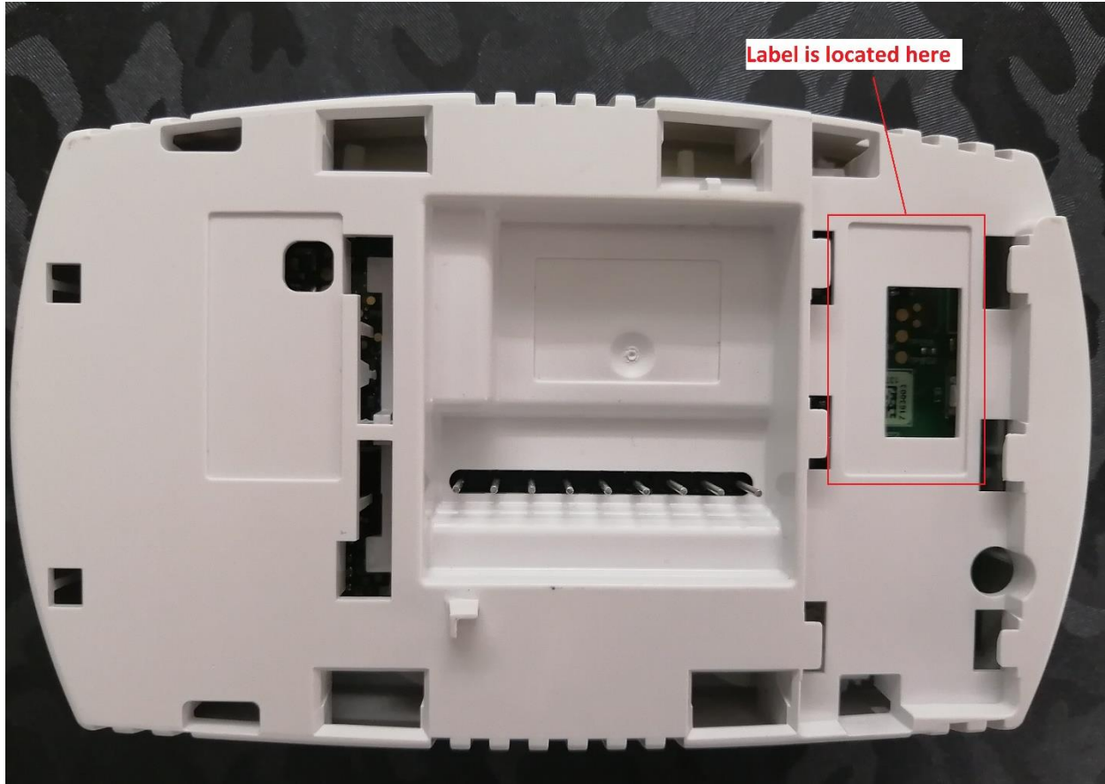
Figure 1. Back side of thermostat – FCC/ISED Label location.
