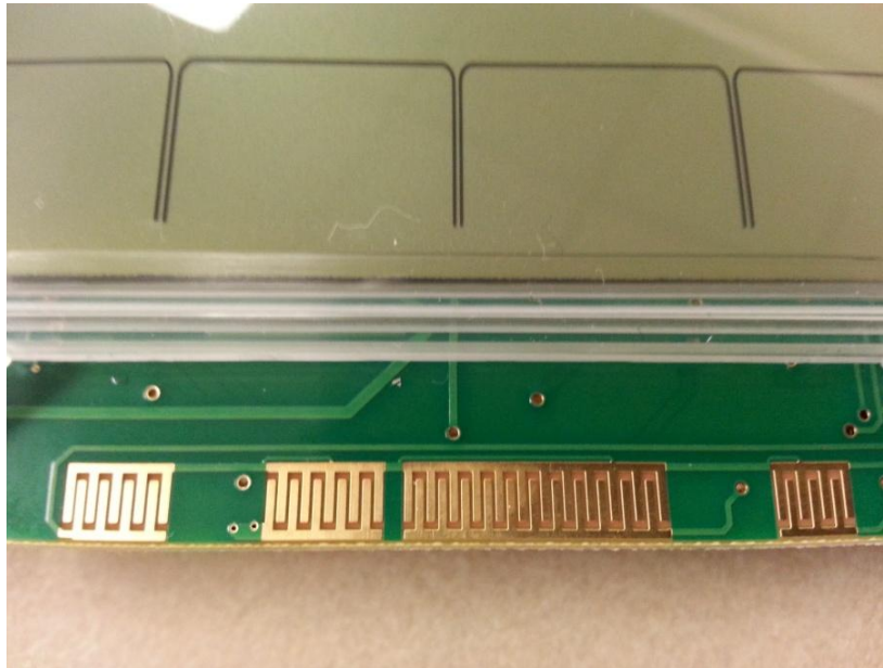
Close Up # 3 - Portion of Back Side of Board
