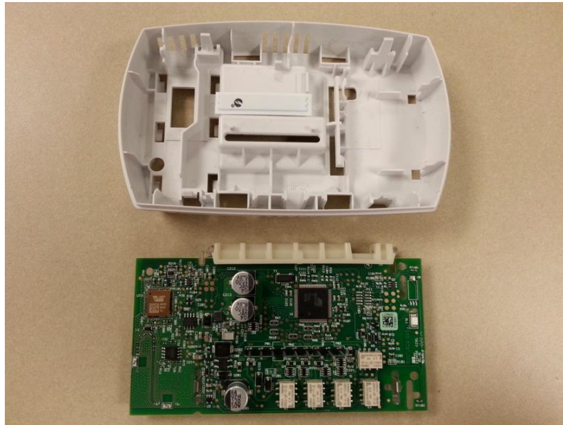
Open for Inspection – RF Section
