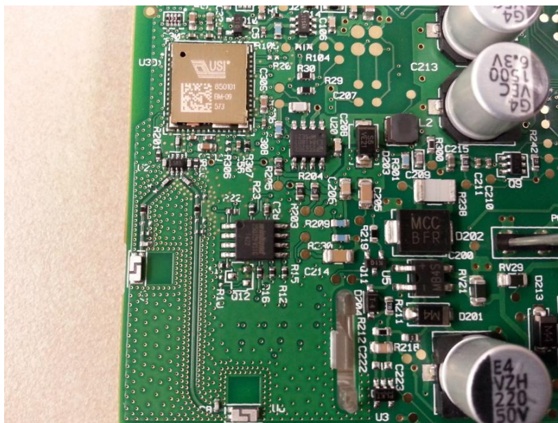
Board – Close Up of RF Section, View # 1
