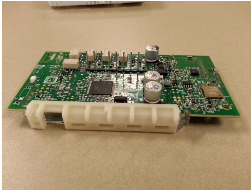
Board – RF Section View # 3
