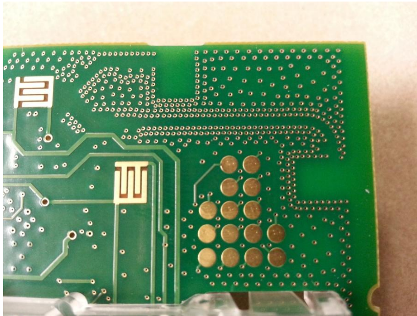
Close Up # 1 - Portion of Back Side of Board
