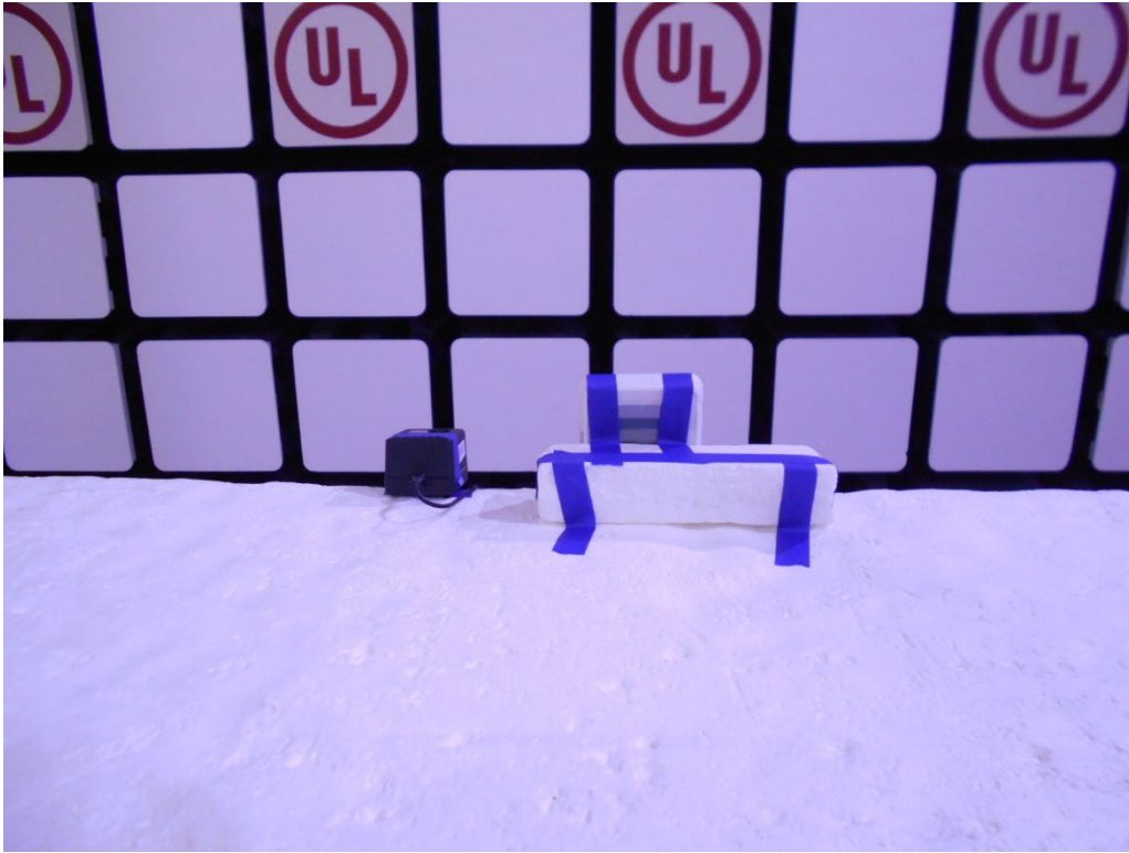
RADIATED 18-26 GHz FRONT
