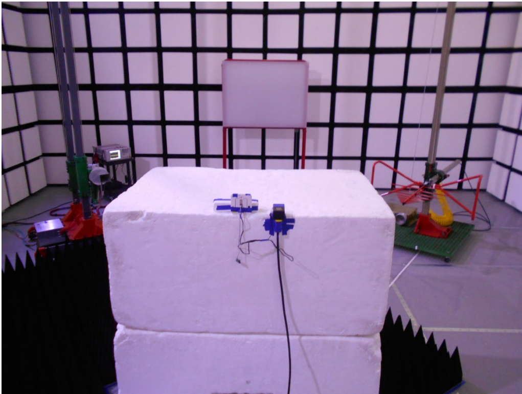
RADIATED 18-26 GHz BACK
