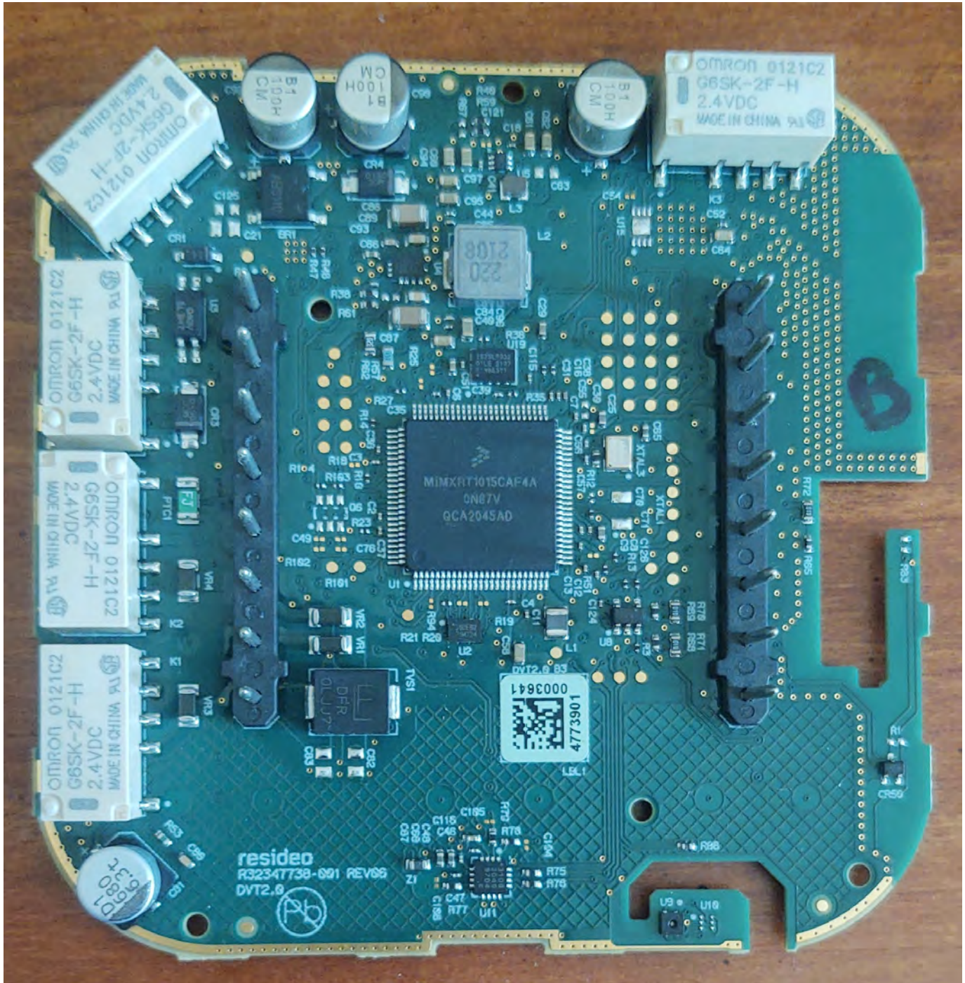
Figure 2. Bottom Layer.
