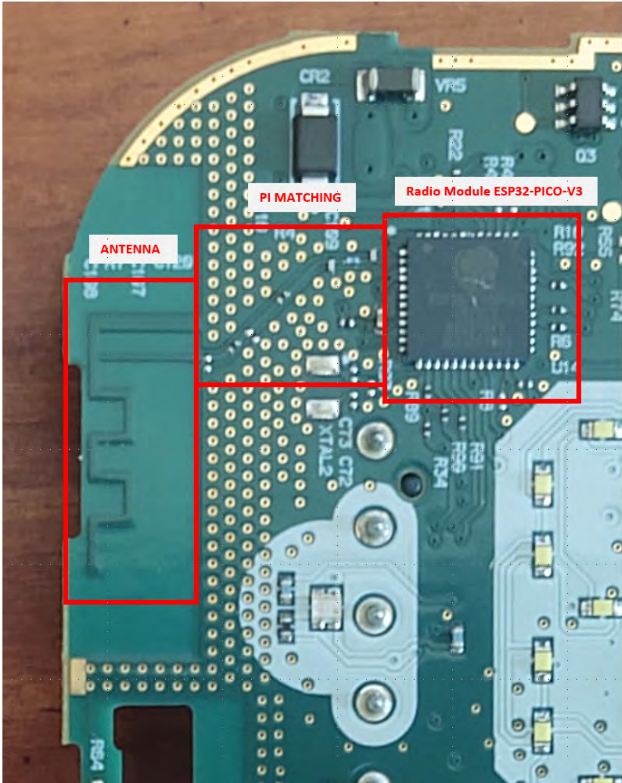
Figure 3. RF Section.
