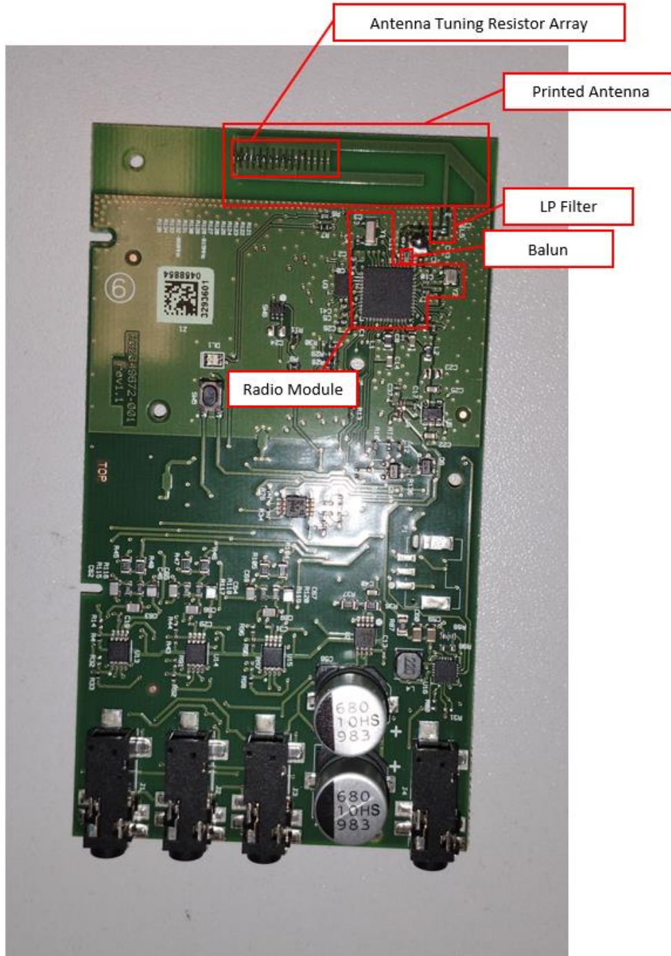
Figure 3. RF circuit identification.
