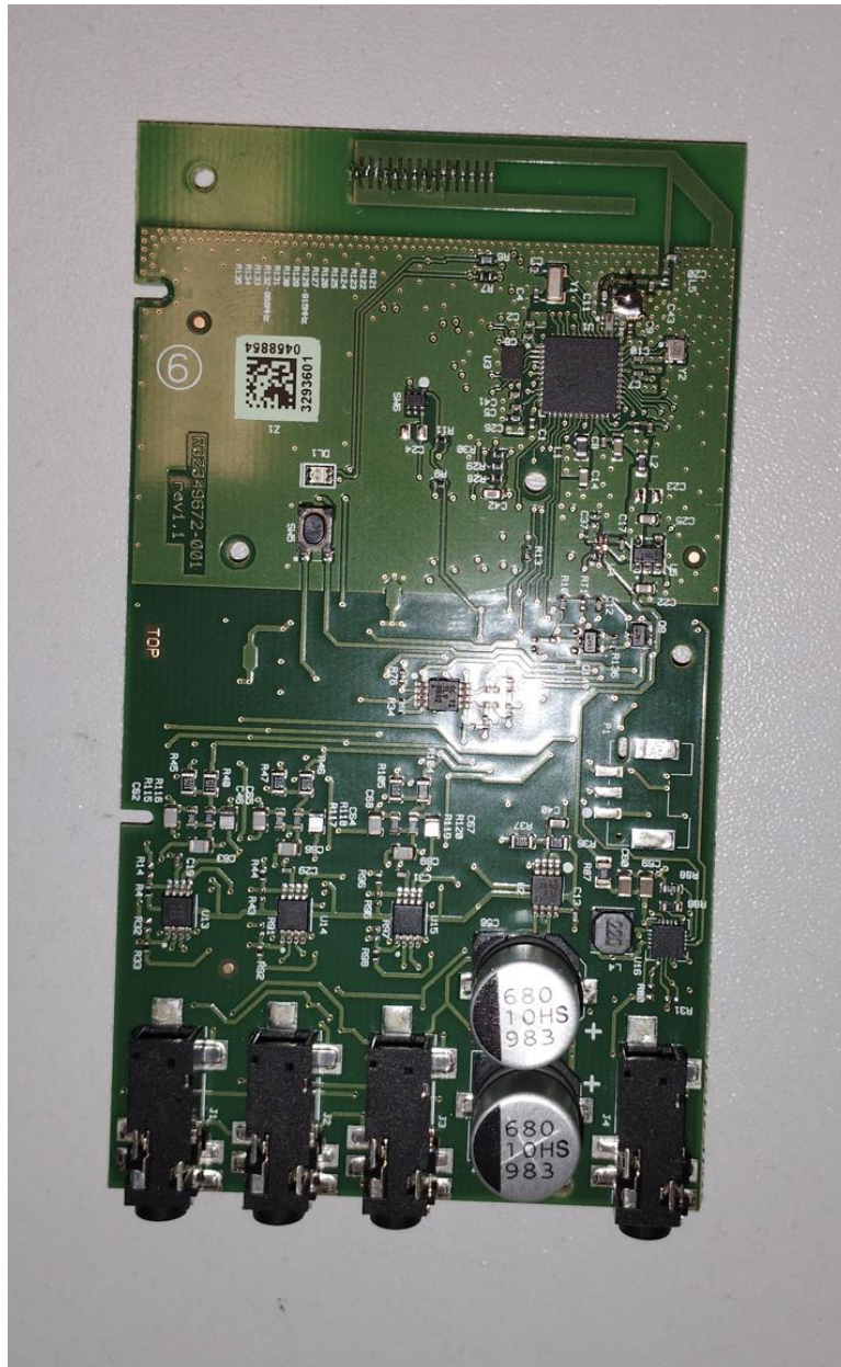
Figure 1. PCB Top side view.
