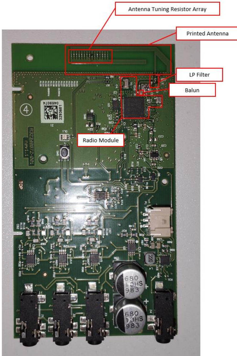
Figure 3. RF circuit identification.
