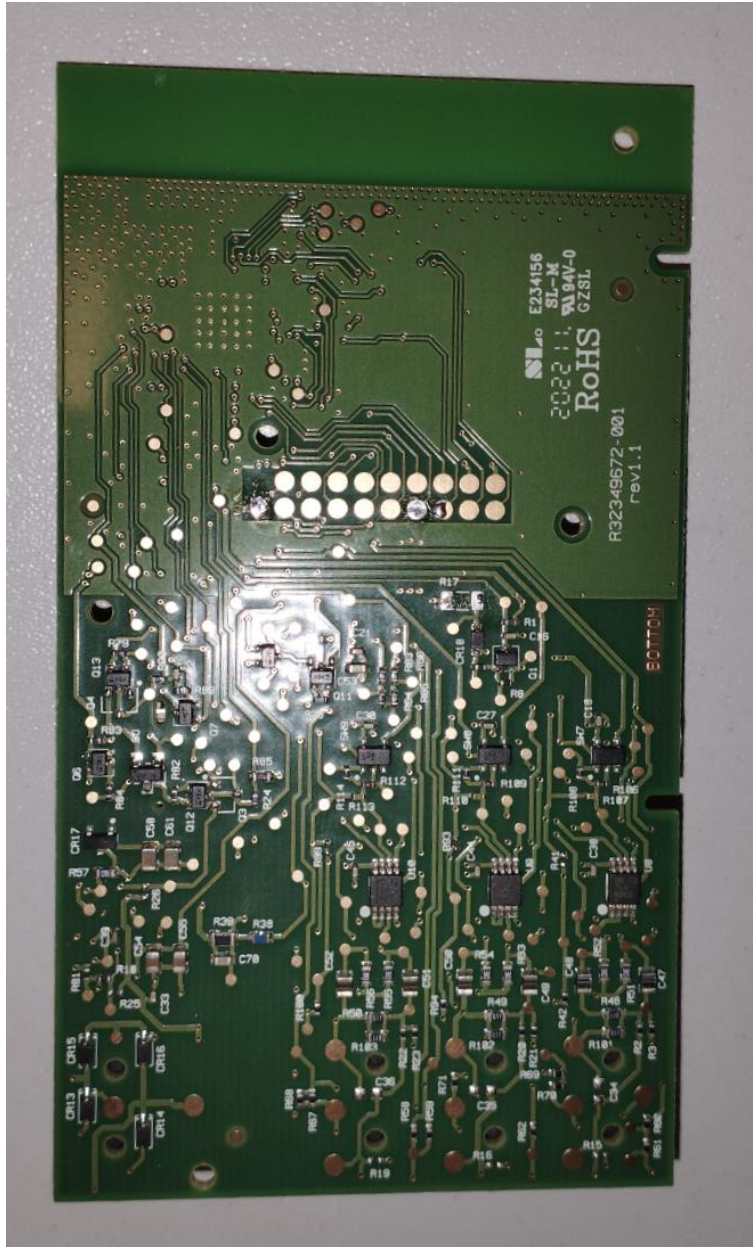
Figure 2. PCB Back side view.
