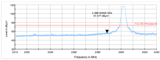
BLE Channel 0 Peak
