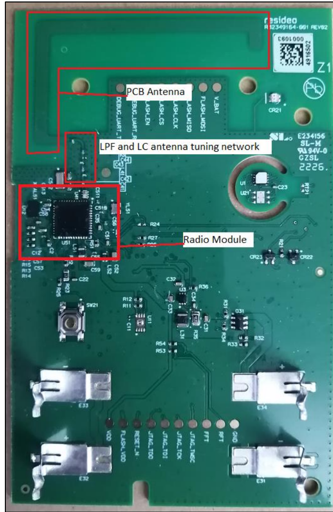
Figure 3. RF circuit identification.
