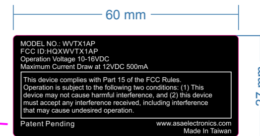
FCC ID label LC2-1209002-1R
