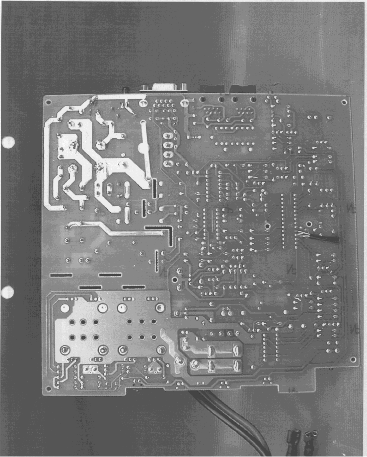
PHOTO 12. EUT SOLDERING SIDE VIEW (MBK 520)
