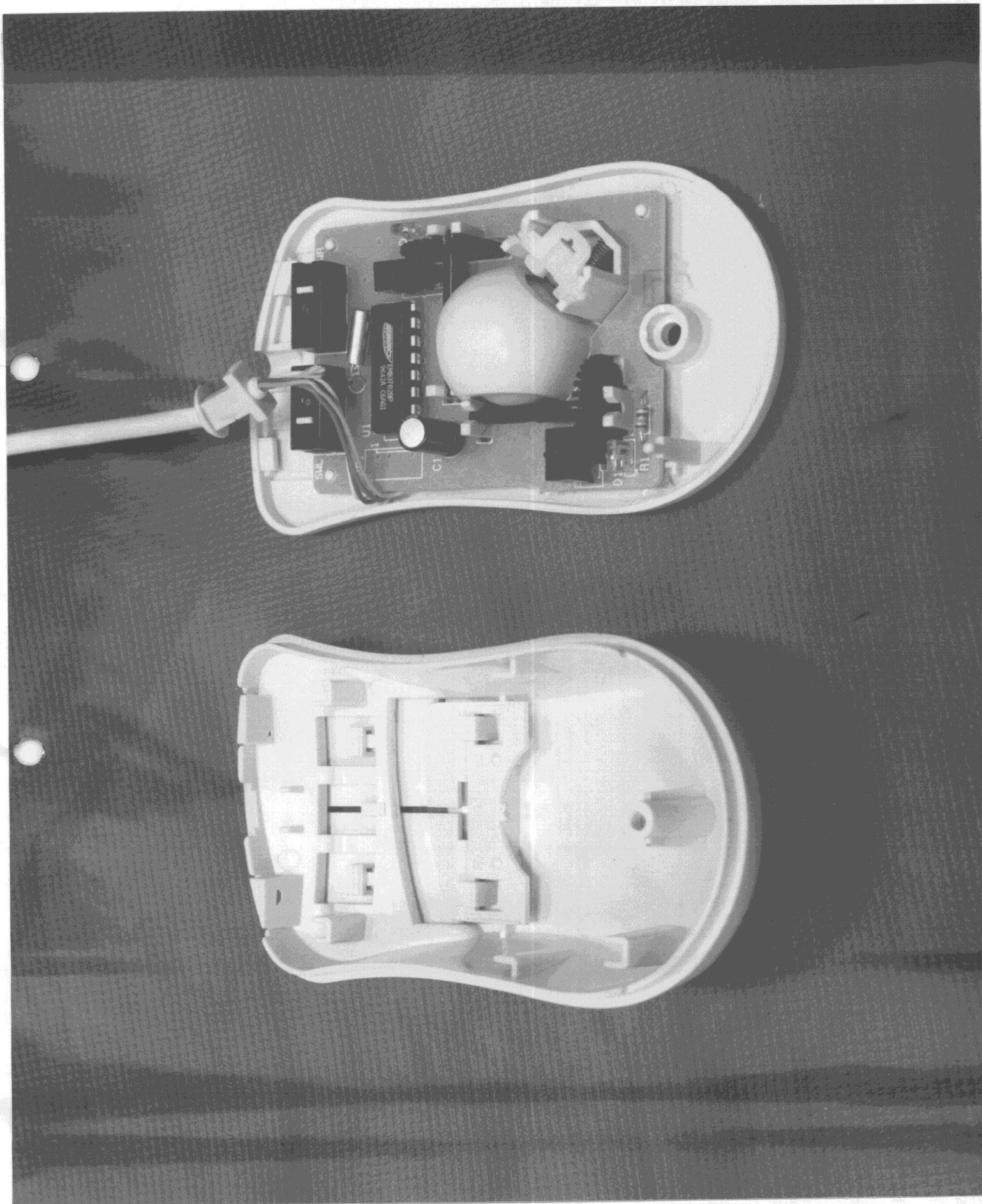
FCC ID : HOXPC97010-68 PHOTO 3. EUT INSIDE VIEW
