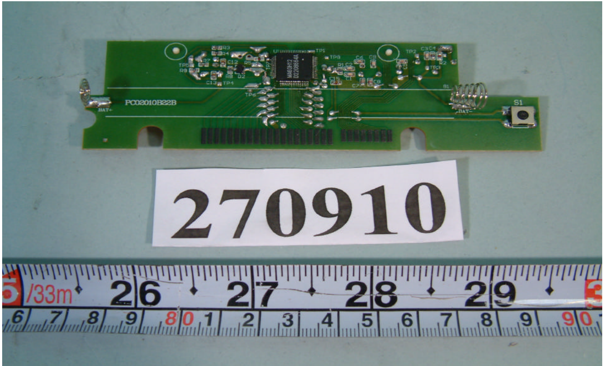
REAR side of Main Board Of Keyboard
