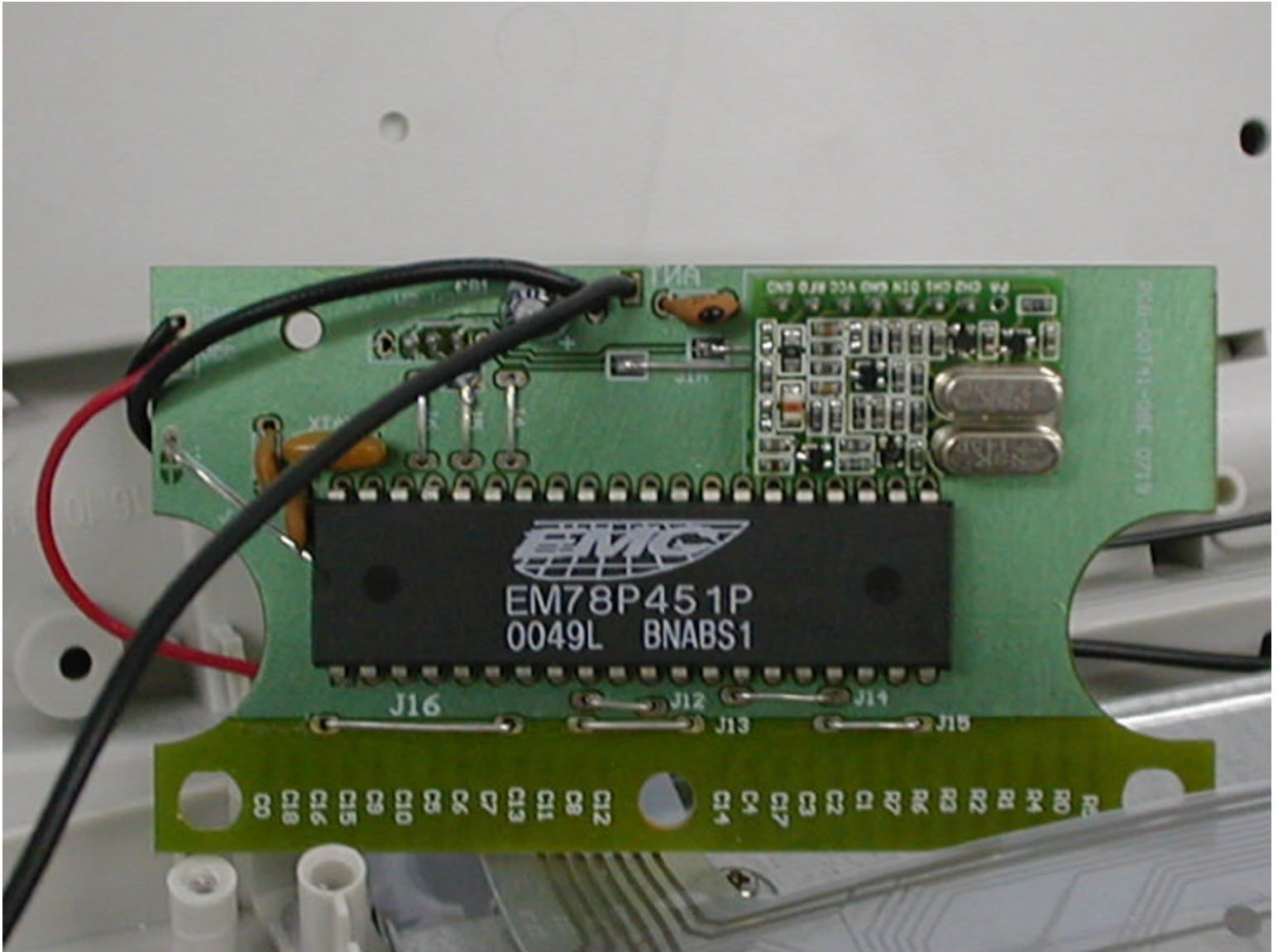
01R9829 Transmitter
