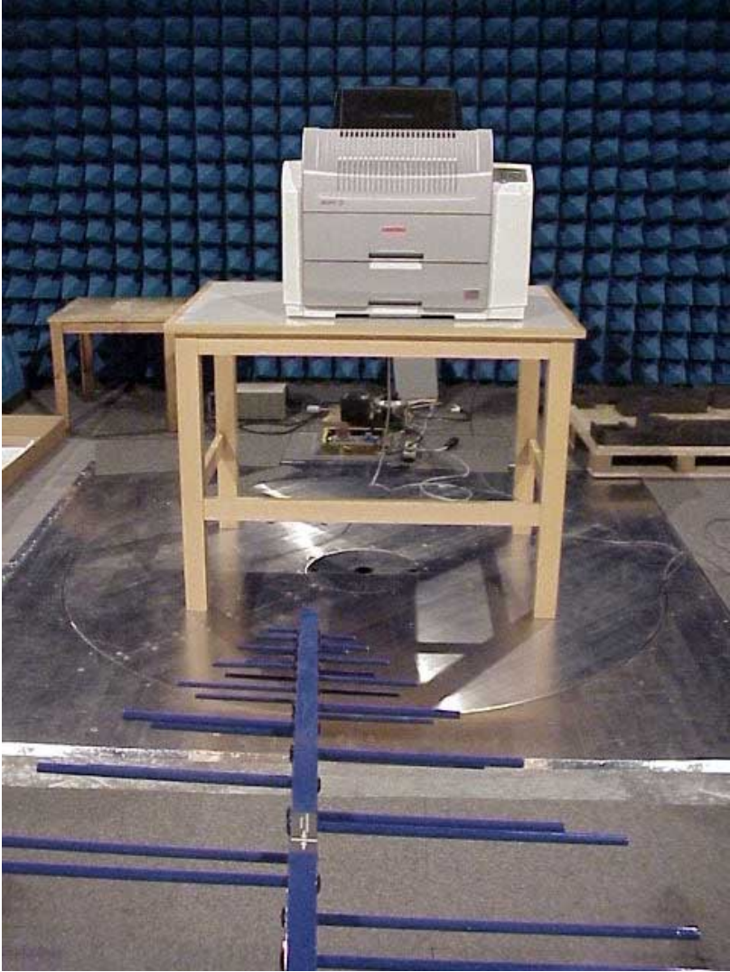
photo 2: radiated emission set-up (30-1000MHz)
