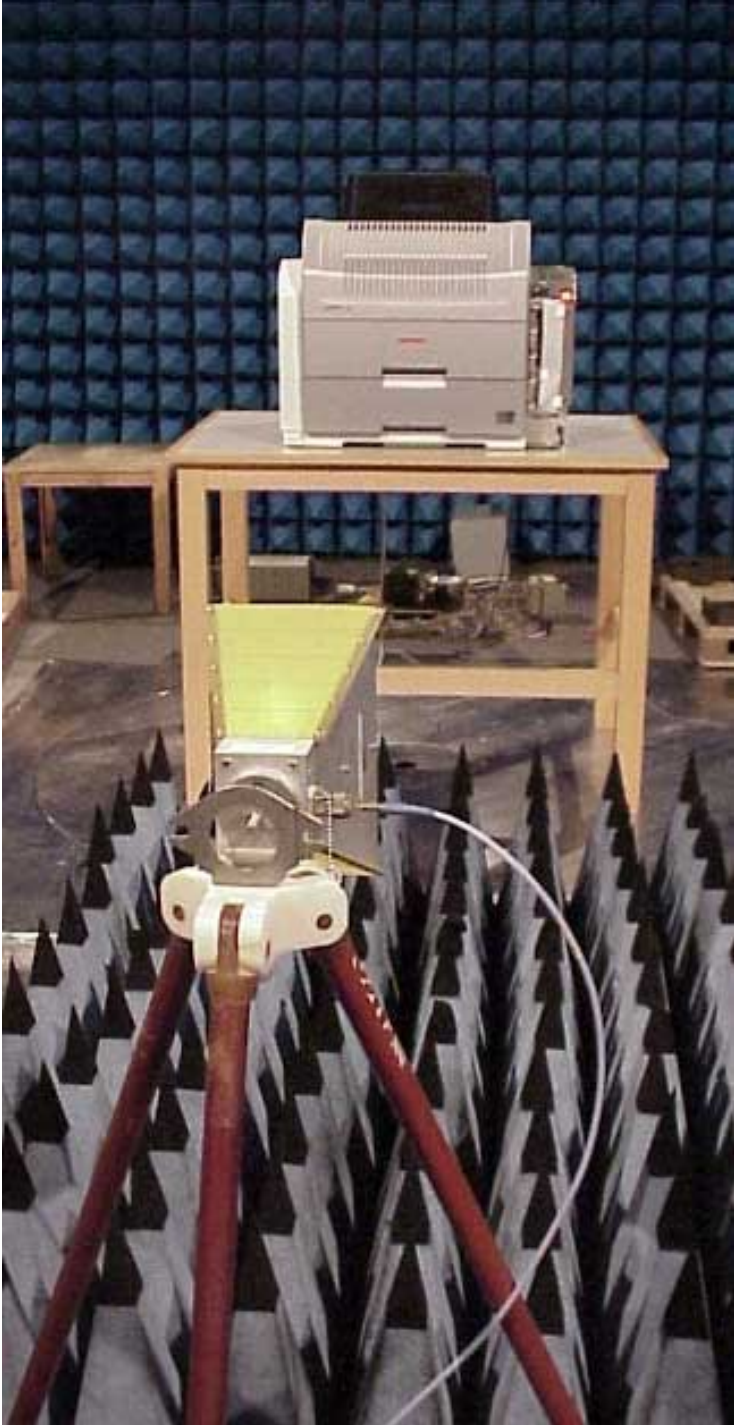
photo 3: radiated emission set-up (1-5GHz)
