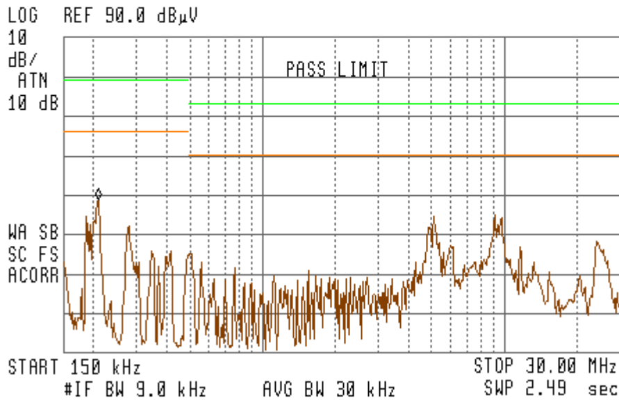
6.2 fig2 Conducted emission L2-PE (115V/60Hz)
