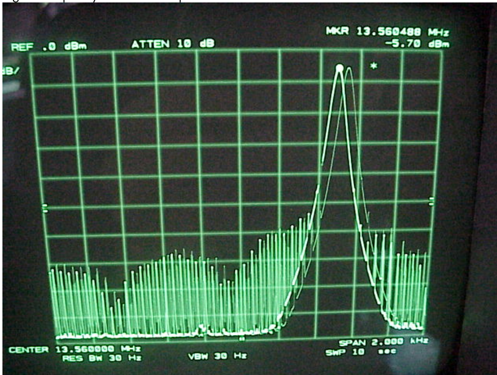
Fig 8 : frequency deviation temp .
