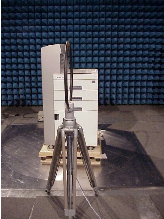
Photo 7 : fundamental radiated emission (ISM 13.65MHz)
