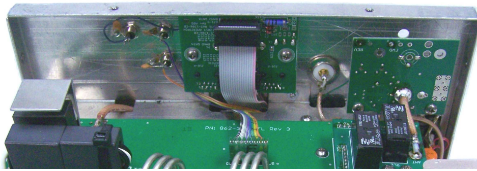
ALS-1406 Back Panel with RJ45 Board and SWR Board
