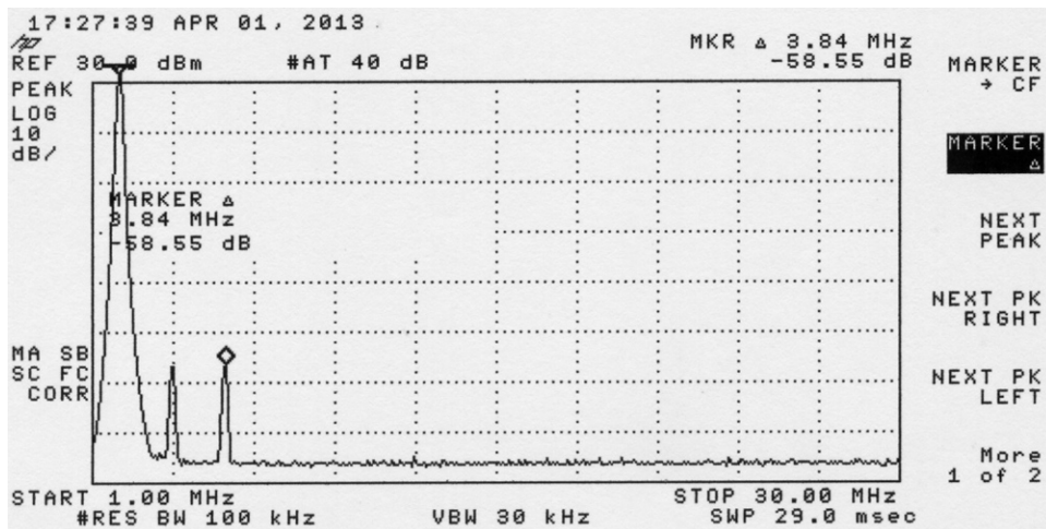
1.96 MHz 3 rd harmonic -59 dB @1200W
