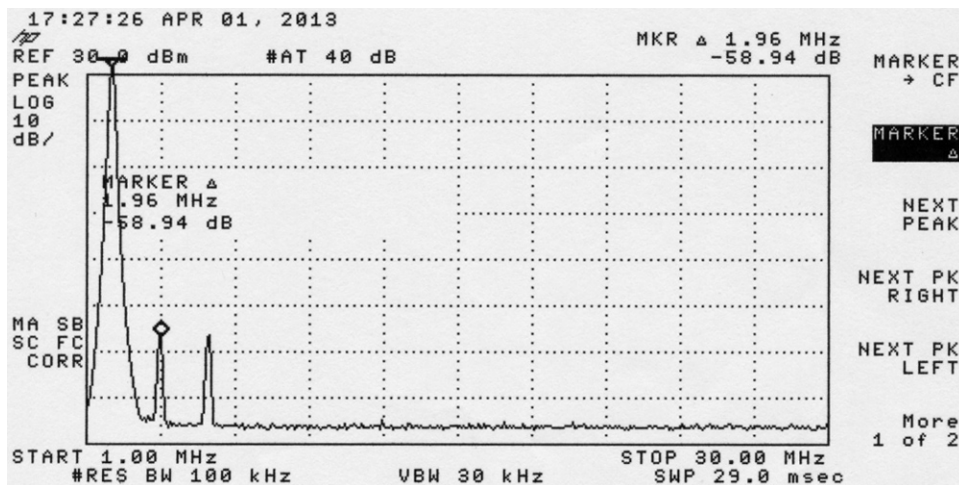
1.96 MHz 2 nd harmonic -59 dB @1200W
