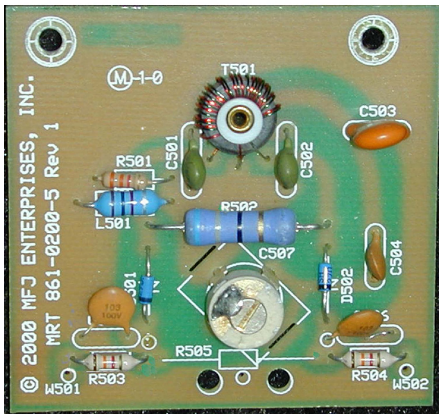
SWR directional coupler
