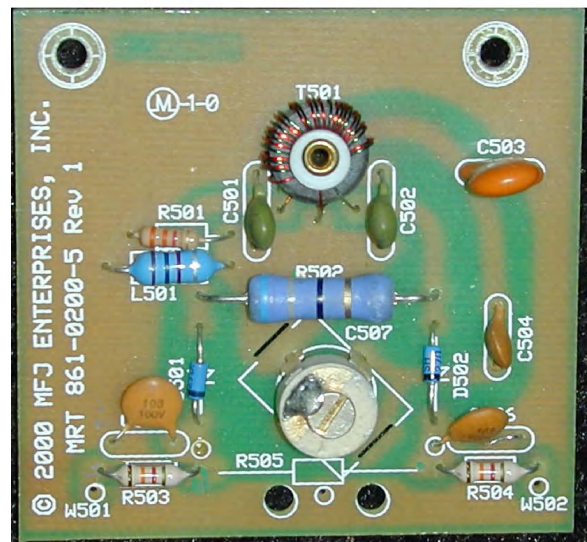
SWR directional coupler
