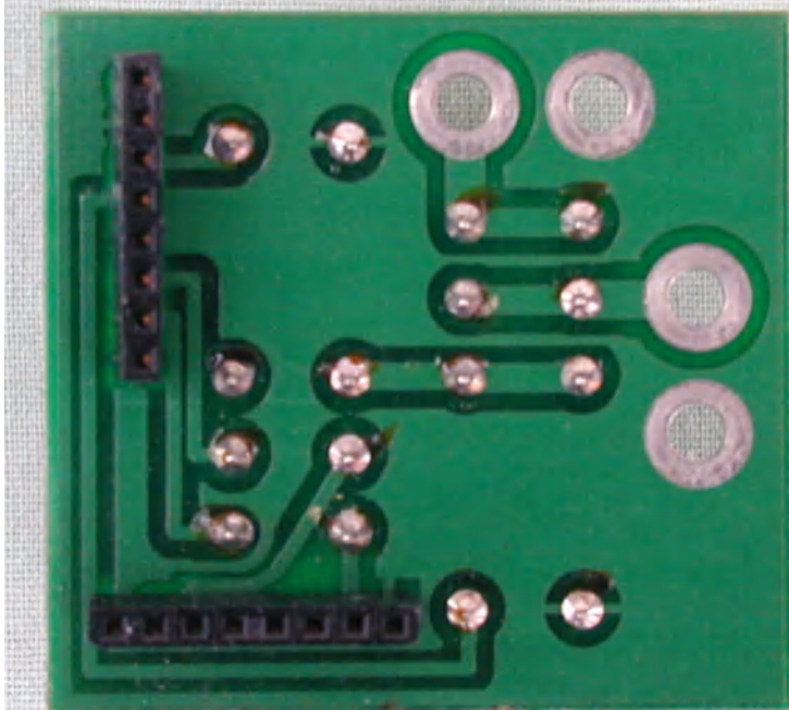
RLY bottom
