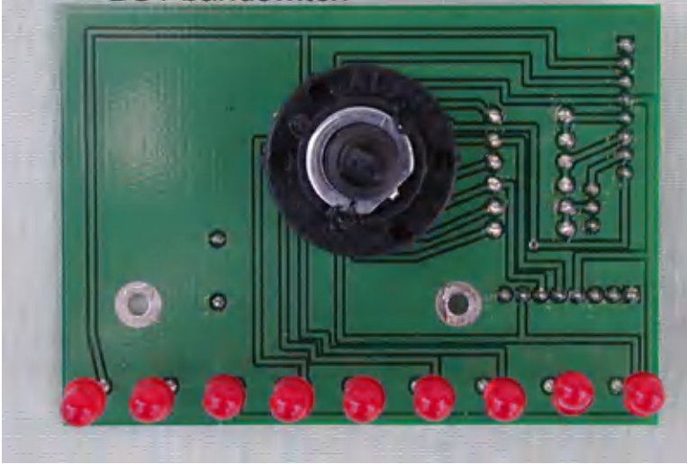
BS1 bandswitch
