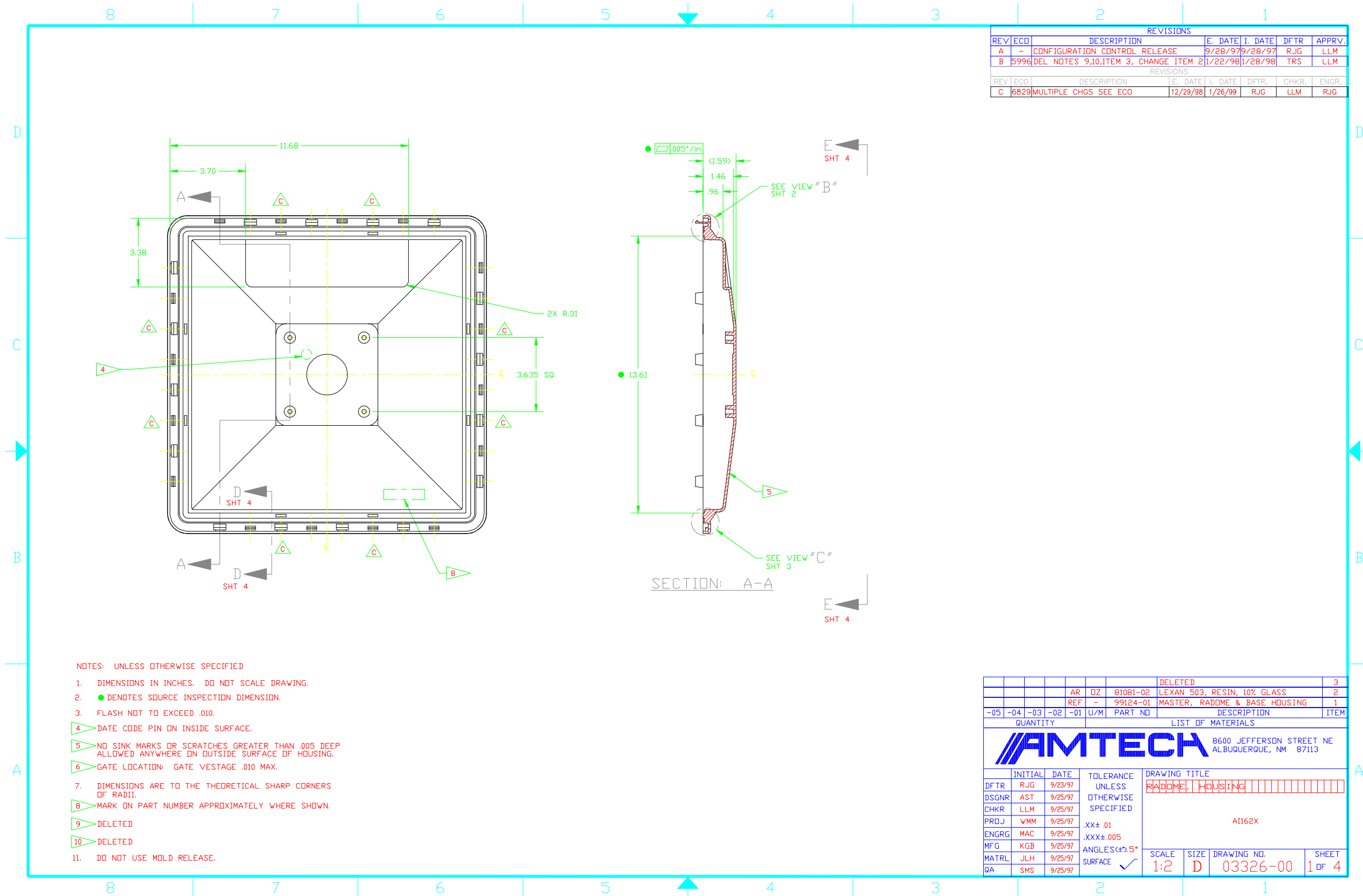
915 MHz Antenna Enclosure, Amtech Systems Division, Intermec Technologies Two pieces snap together to form complete enclosure.
