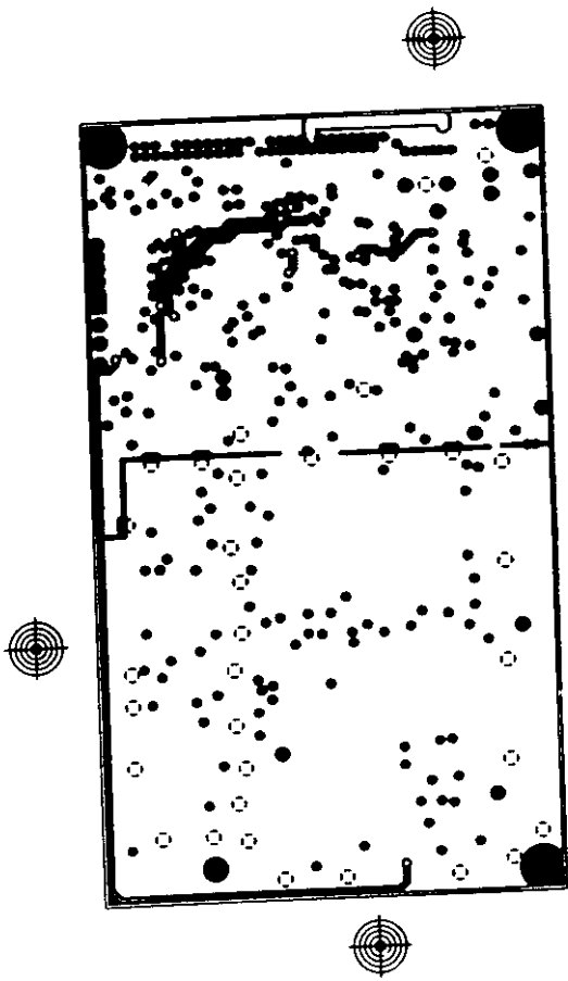
GROUND PLANE LAYER 2
