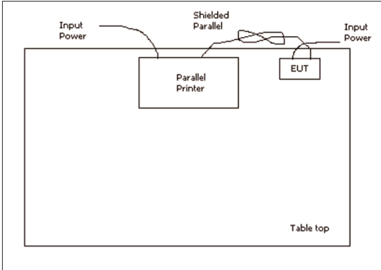
Conducted Emissions
