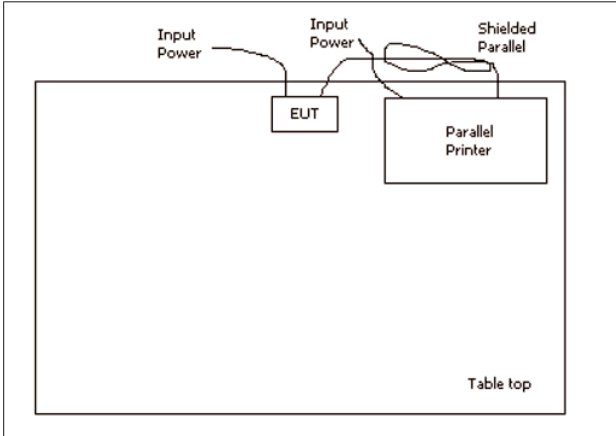
Radiated Emissions
