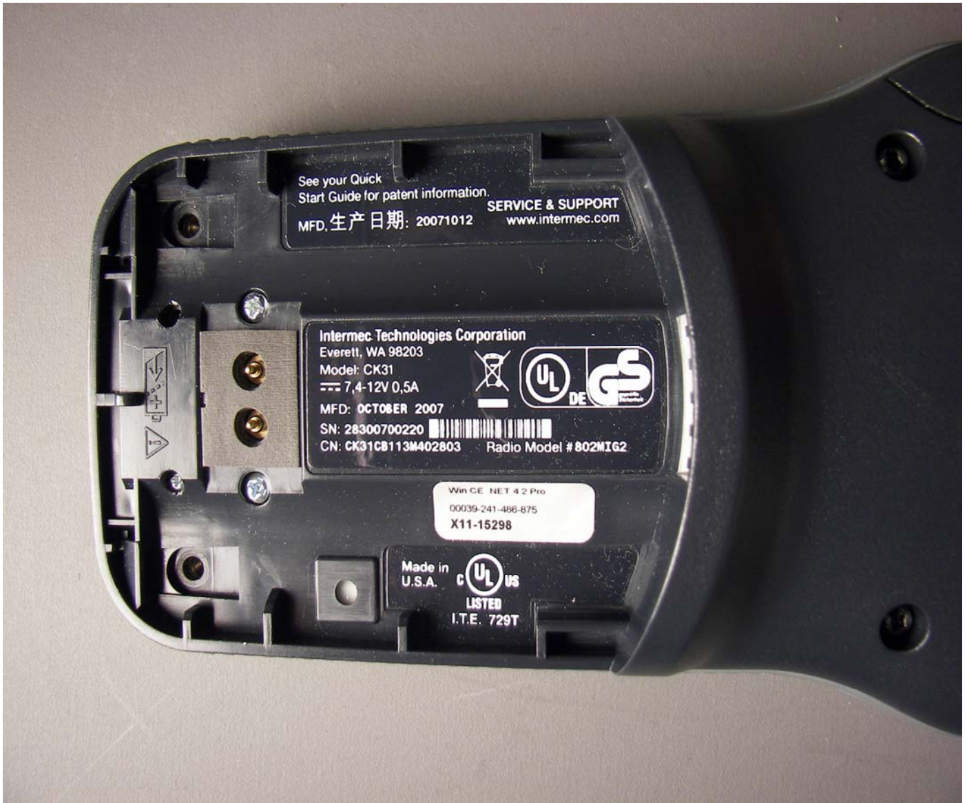
CK31 – back view. Battery compartment labeling.
