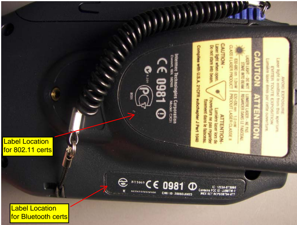
CK31 (Large Back) – back view. Labeling.
