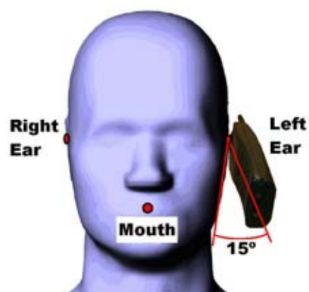
Figure 16. – 15° Tilt Position.
