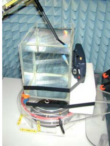
Figure 52. Positional photograph of 700C-SMC45 in the alternative 0.0mm Touch Position
