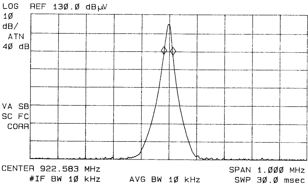
Figure 9 Antenna Conducted Emissions
