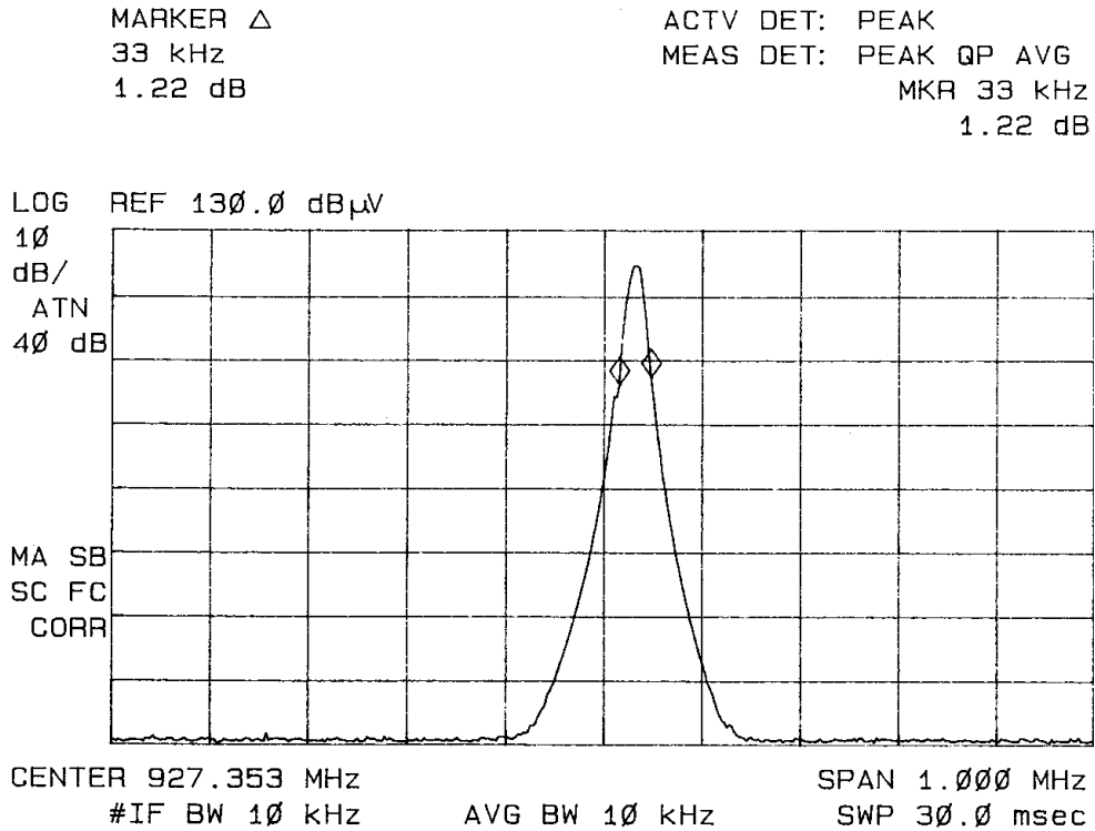
Figure 10 Antenna Conducted Emissions
